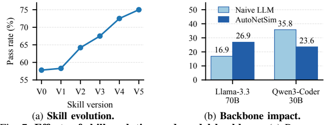
Fig. 7: Effects of skill evolution and model backbone. (a) Pass-rate improvement across accepted skill versions. (b) Pass rates of Naive LLM and AutoNetSim with two open-source backbones.
