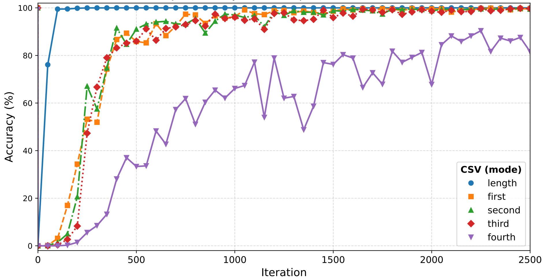
Joint accuracy vs iteration (positions [1, 2, 3, 4])
