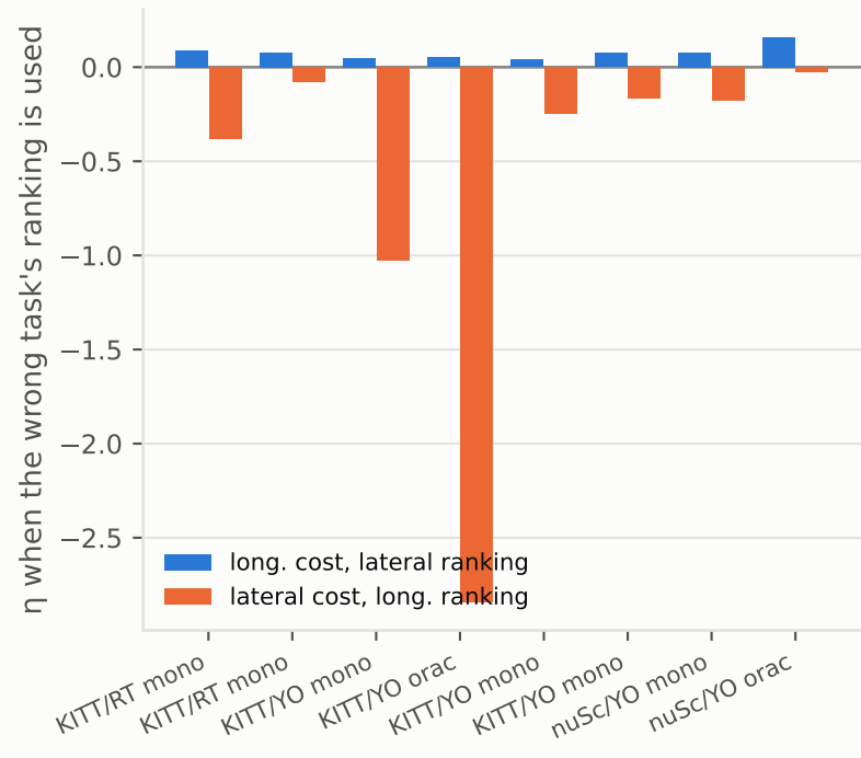
C Cross-applying a ranking is harmful
