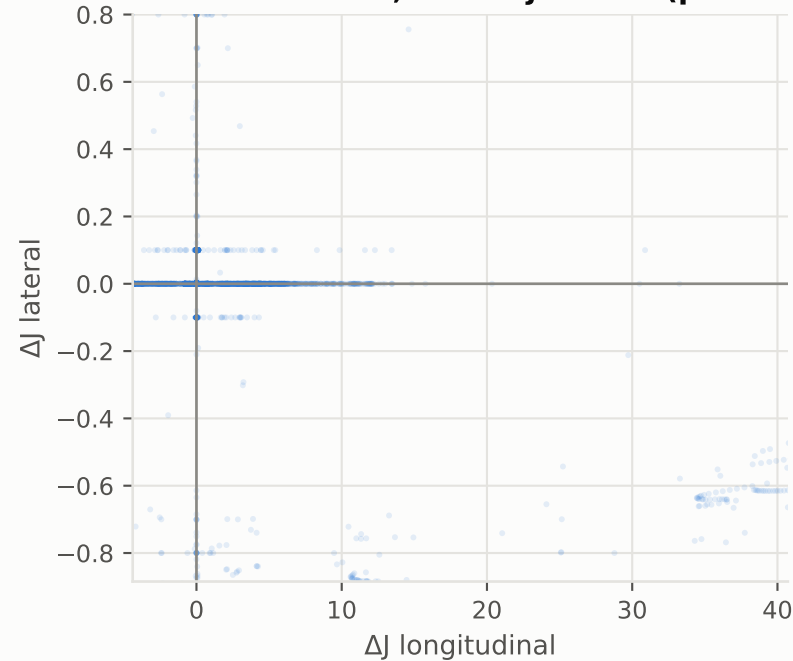
A Same frames, two objectives ( \rho=-0.136 )
