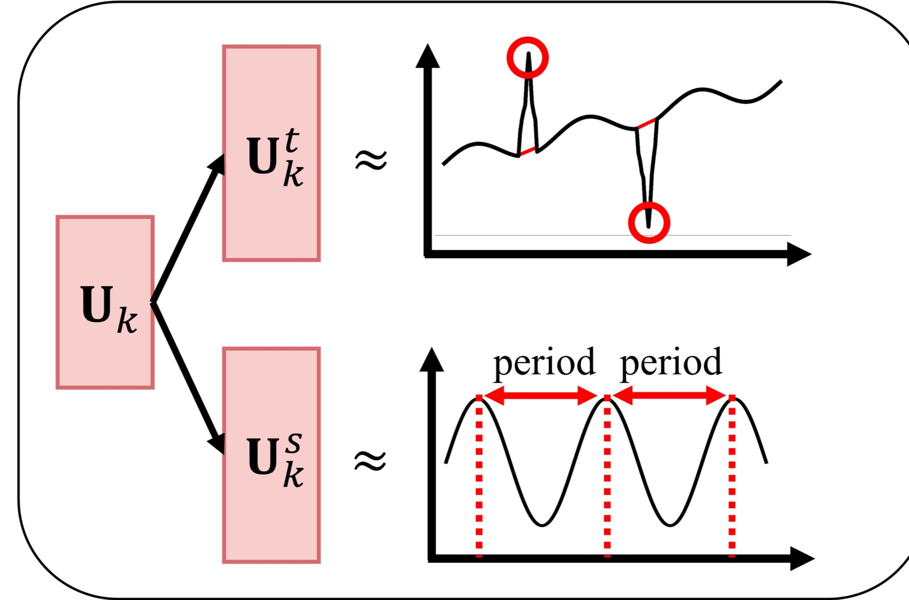
(b) Separation and Regularization
