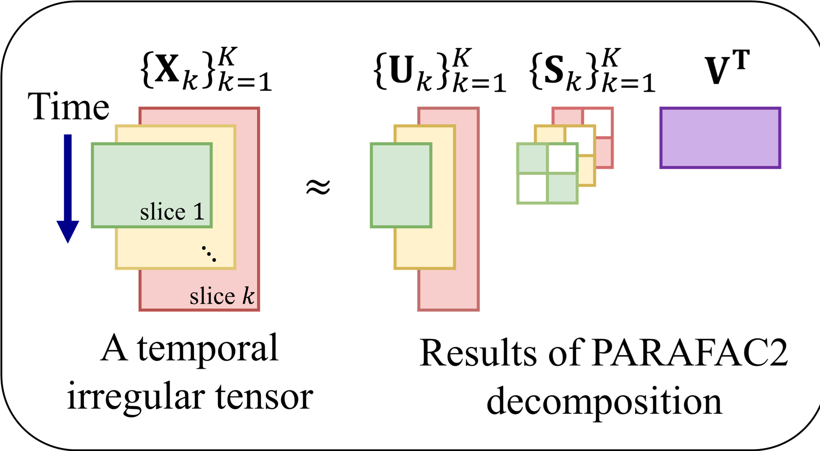
(a) PARAFAC2 Decomposition
