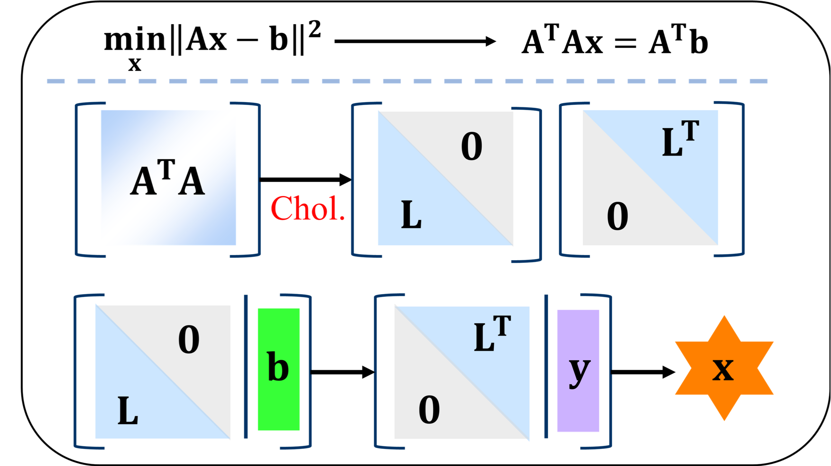
(c) Cholesky-based Optimization
