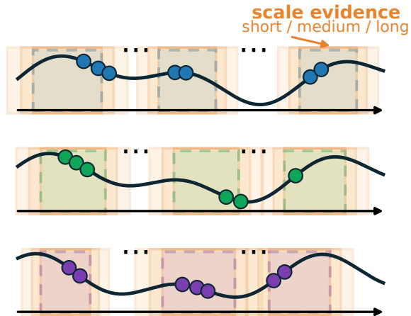
(b) Multi-scaled Patching
