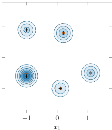
PALM ( s = 6 )
