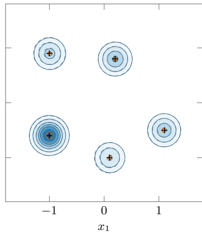
VarPro ( s = 5 )
