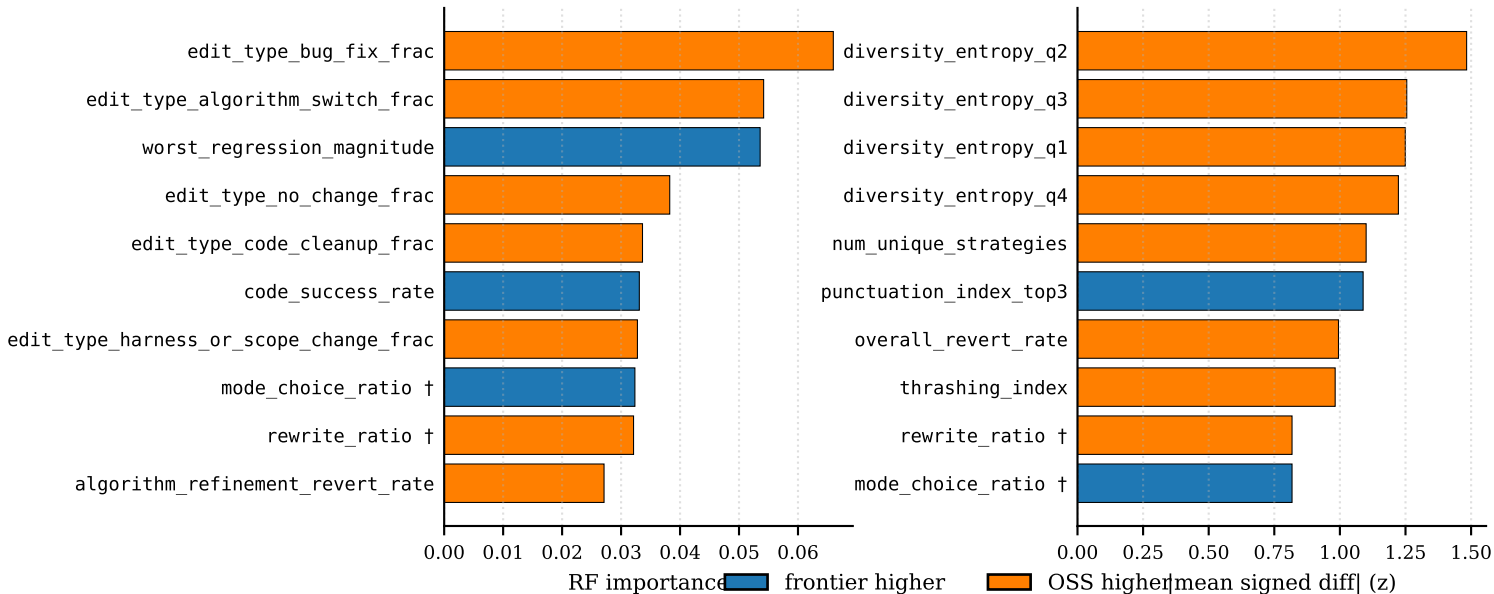
(a) full-profile classifier (60 features)
