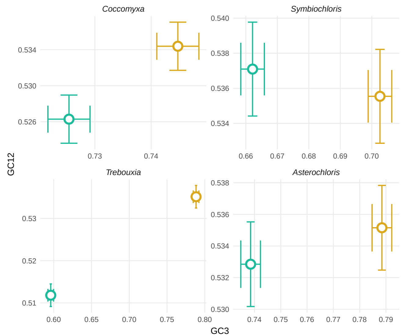
Neutrality Plot: GC12 vs GC3
