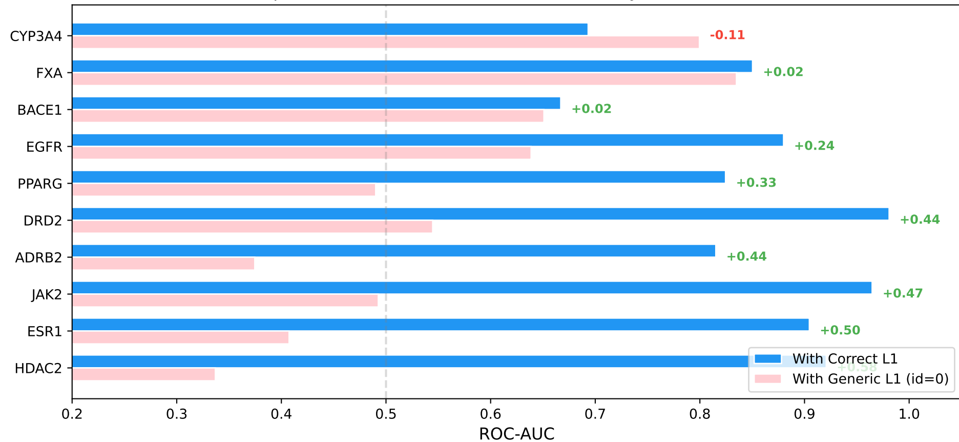
V2-Expanded: "Broken" Model Rehabilitated by Correct L1 Context
