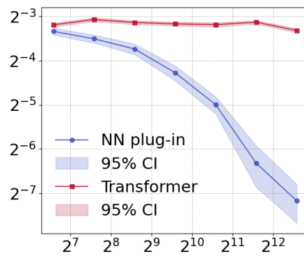
Figure 3: Classifier comparison between NN-based plug-in and Transformer.
