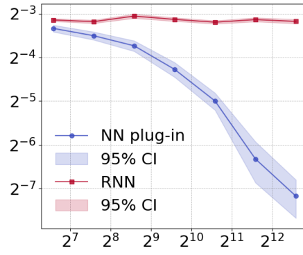
Figure 1: Classifier comparison between NN-based plug-in and RNN.
