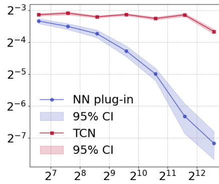
Figure 2: Classifier comparison between NN-based plug-in and TCN.
