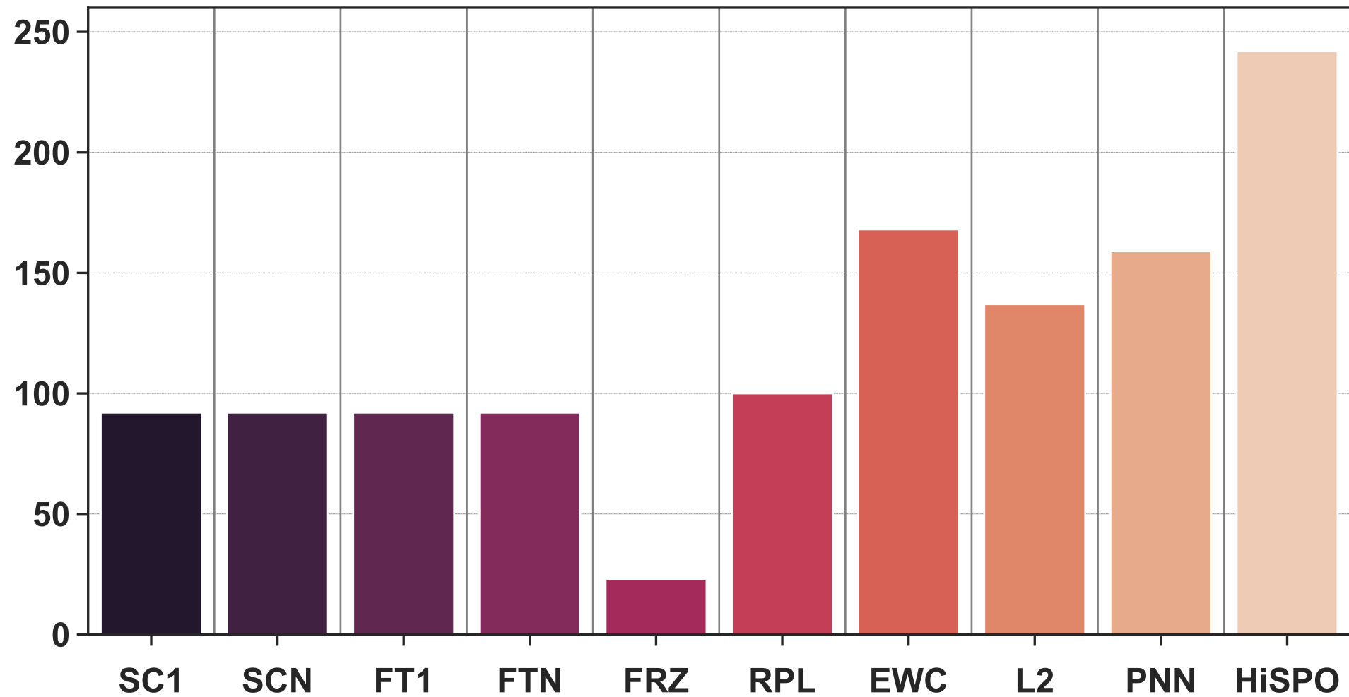
Training Time ( in min )
