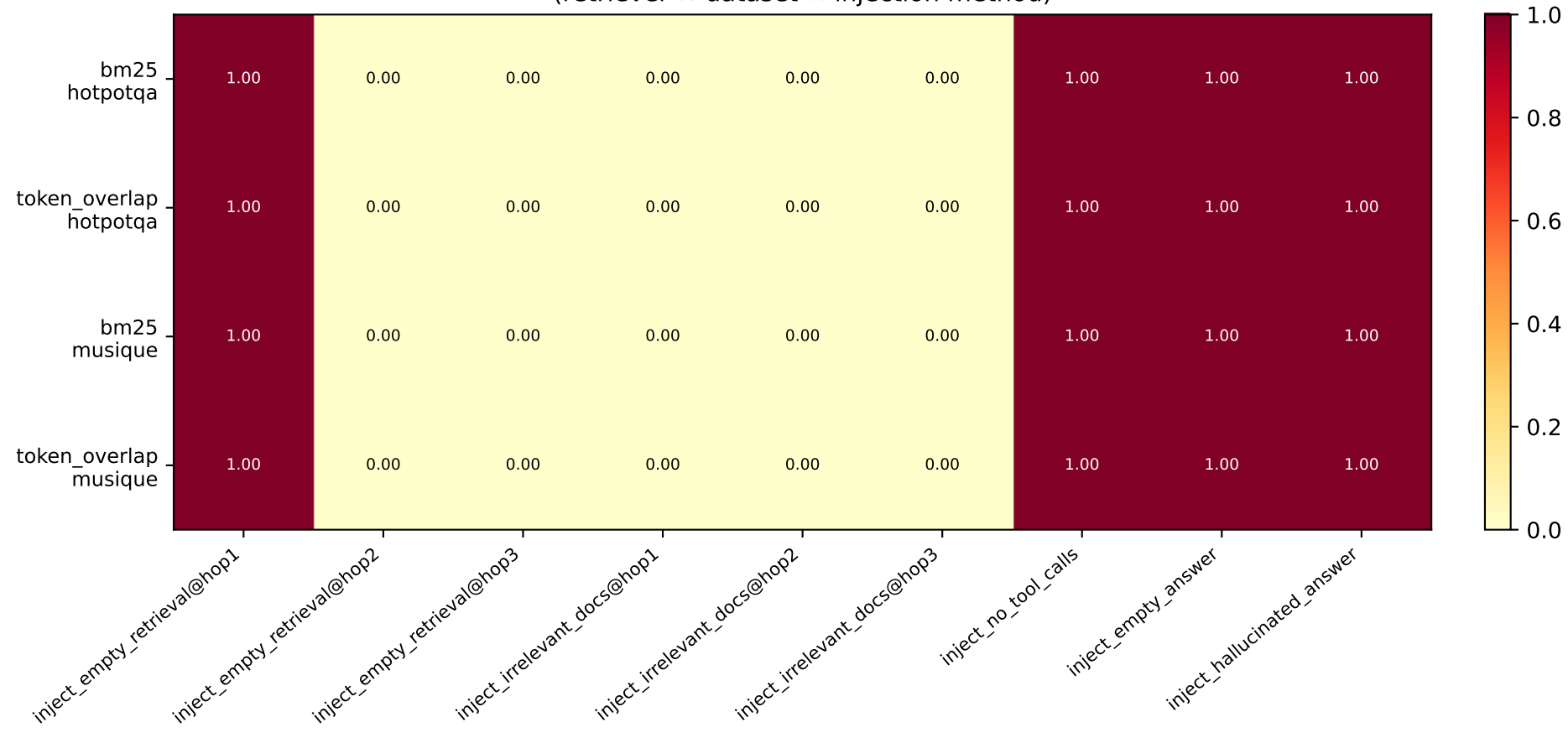
Benchmark Table — Root-Cause Accuracy (retriever × dataset × injection method)
