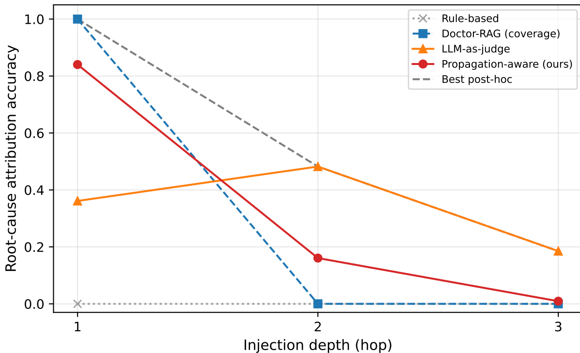
Attribution identifiability — claude:claude-haiku-4-5 · frames (n_failed=[119, 116, 123]; recovery=[0.26, 0.28, 0.23]) PA-LLM-judge \Delta by depth: [0.479, -0.321, -0.176]
