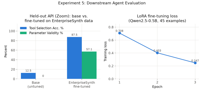
Figure 6: Left: base vs. LoRA-fine-tuned Qwen2.5-0.5B-Instruct on the held-out Zoom eval set. Right: training loss across the 3 fine-tuning epochs.
