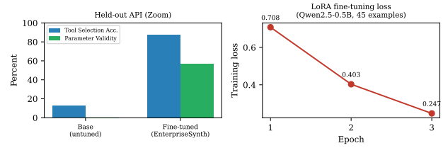
Figure 6: Left: base vs. LoRA-fine-tuned Qwen2.5-0.5B-Instruct on the held-out Zoom eval set. Right: training loss across the 3 fine-tuning epochs.
