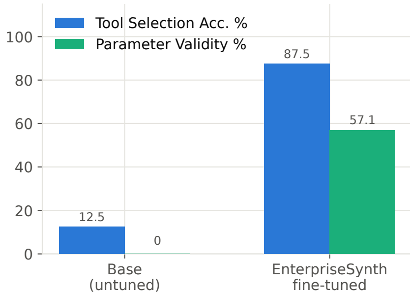
Held-out API (Zoom): base vs. fine-tuned on EnterpriseSynth data
