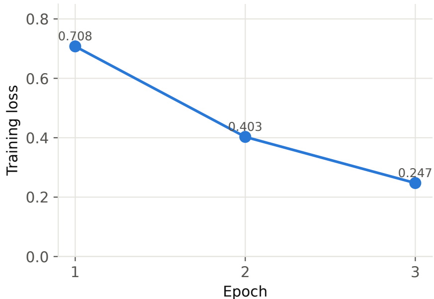
LoRA fine-tuning loss (Qwen2.5-0.5B, 45 examples)
