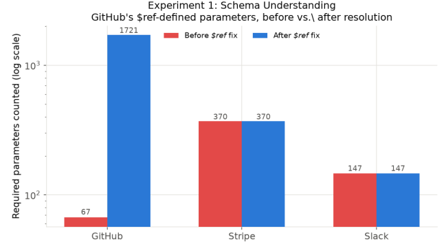
Figure 2: Required-parameter counts before and after the -resolution fix. Stripe and Slack are unaffected; GitHub’s count grows from 67 to 1,721 once shared, ’d parameters are resolved.
