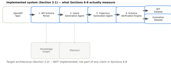
Figure 1: The EnterpriseSynth architecture diagram.
