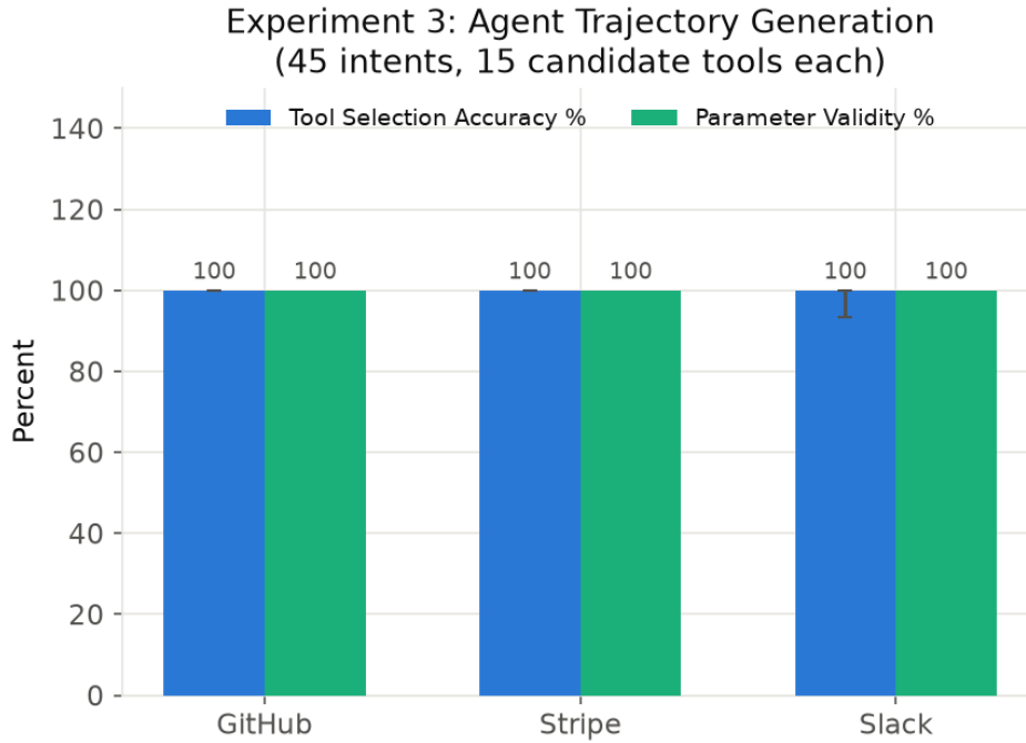
Figure 4: Tool Selection Accuracy and Parameter Validity, 45 intents, 15 candidate tools each. Slack ranged 93.3–100% across repeated runs; see the self-consistency caveat above.
