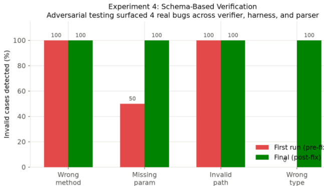
Figure 5: Invalid-case detection rate by corruption type, first run vs. final. Missing-parameter and wrong-type detection were the two categories that required real bug fixes to reach 100%.
