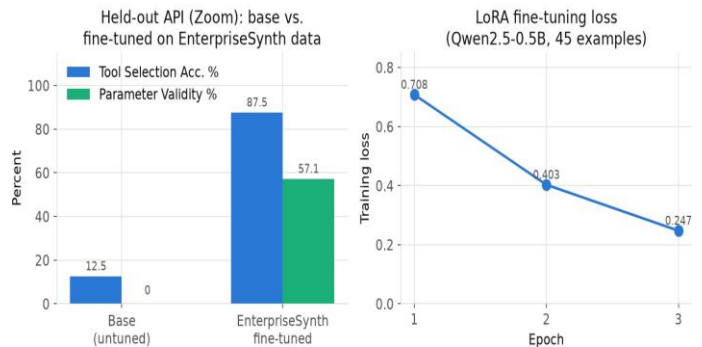
Figure 6: Left: base vs. LoRa-fine-tuned Qwen2.5-0.5B-Instruct on the held-out Zoom eval set. Right: training loss across the 3 fine-tuning epochs.
