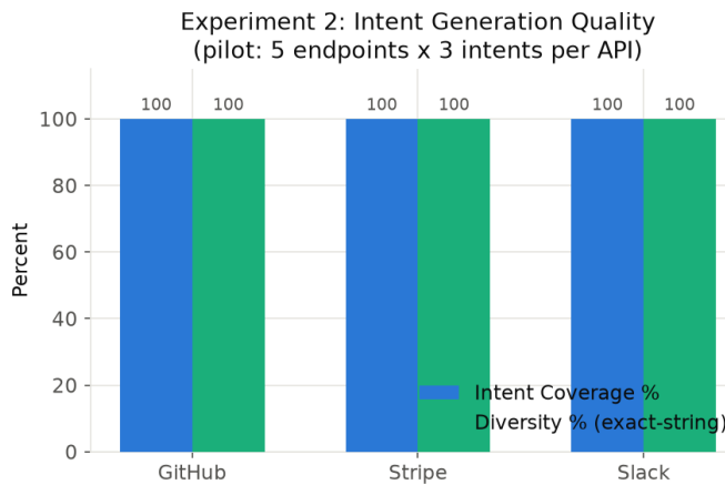
Figure 3: Intent Coverage and exact-string Diversity, 5 endpoints x 3 intents per API. Both flat at 100% annual inspection of the actual generated intents matters more than these aggregates.
