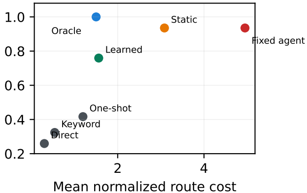
Lexical-shift challenge
