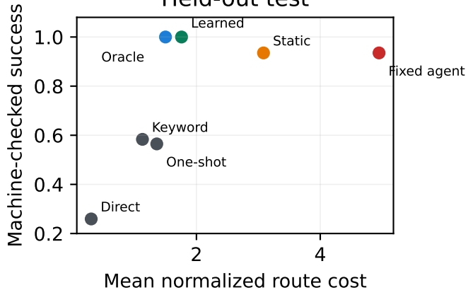
Held-out test
