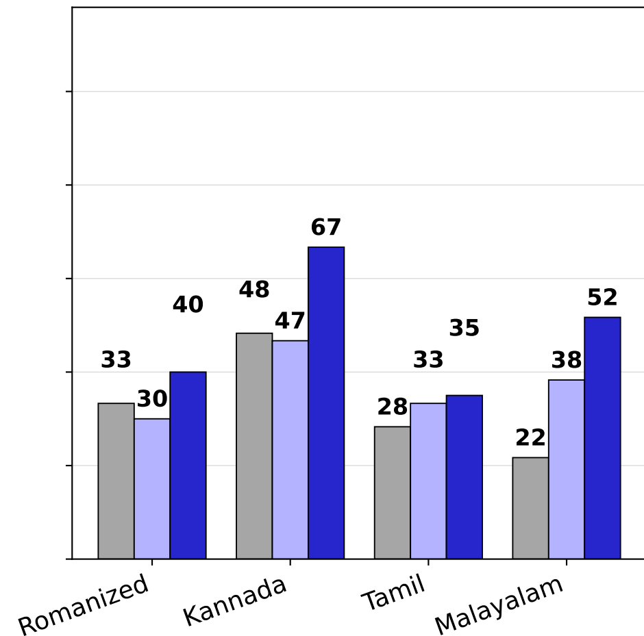
Sarvam
