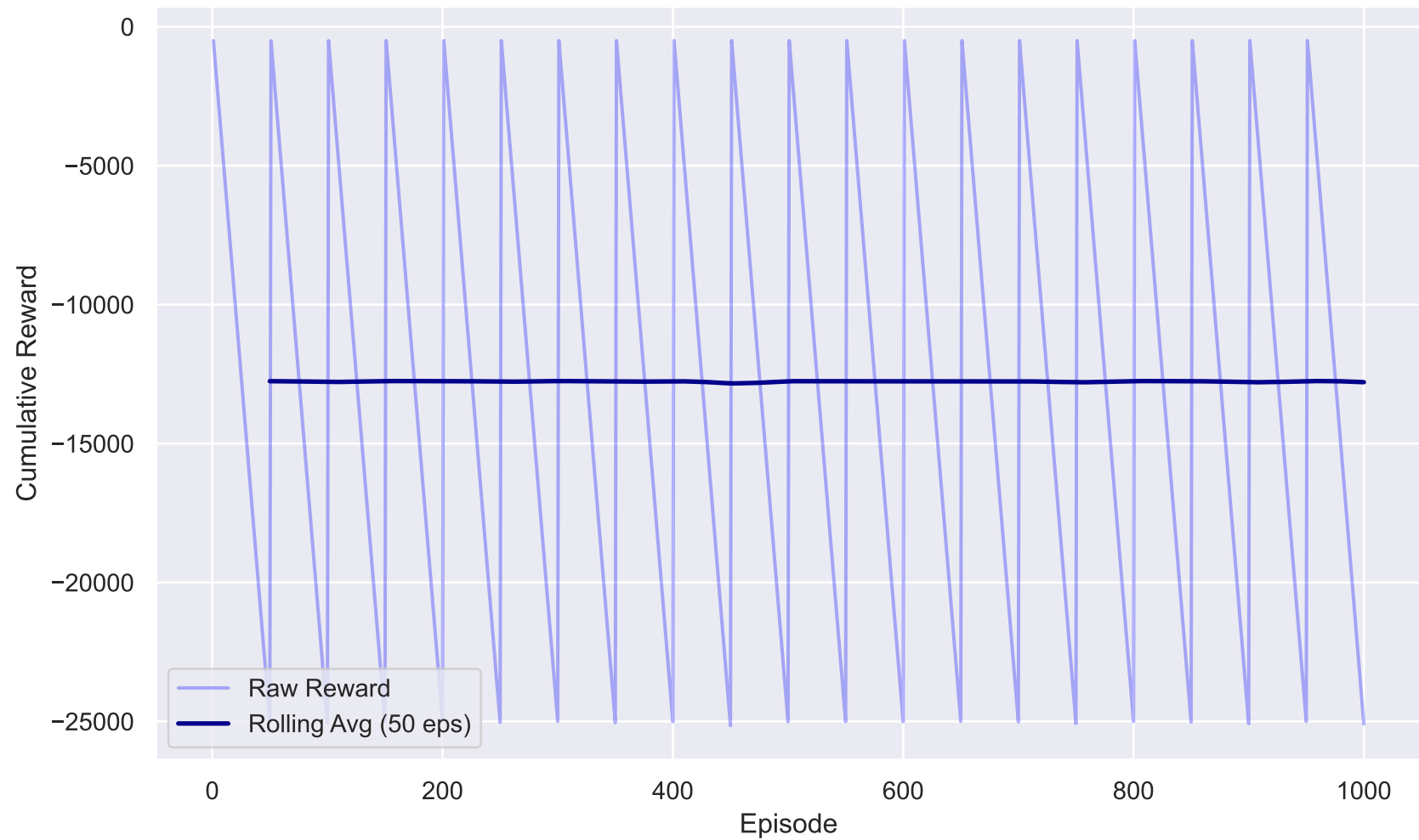
Unlearning Phase: Agent Performance Over Time
