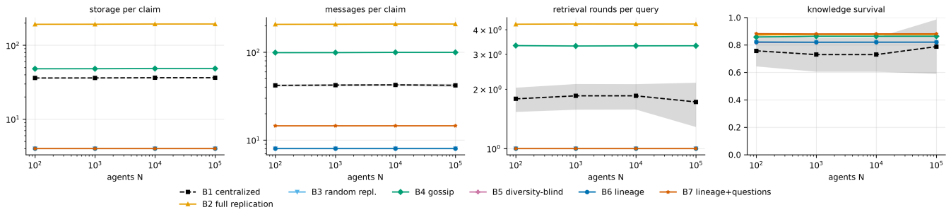
Empirical scaling trend (4 measured scales; not an asymptotic claim)
