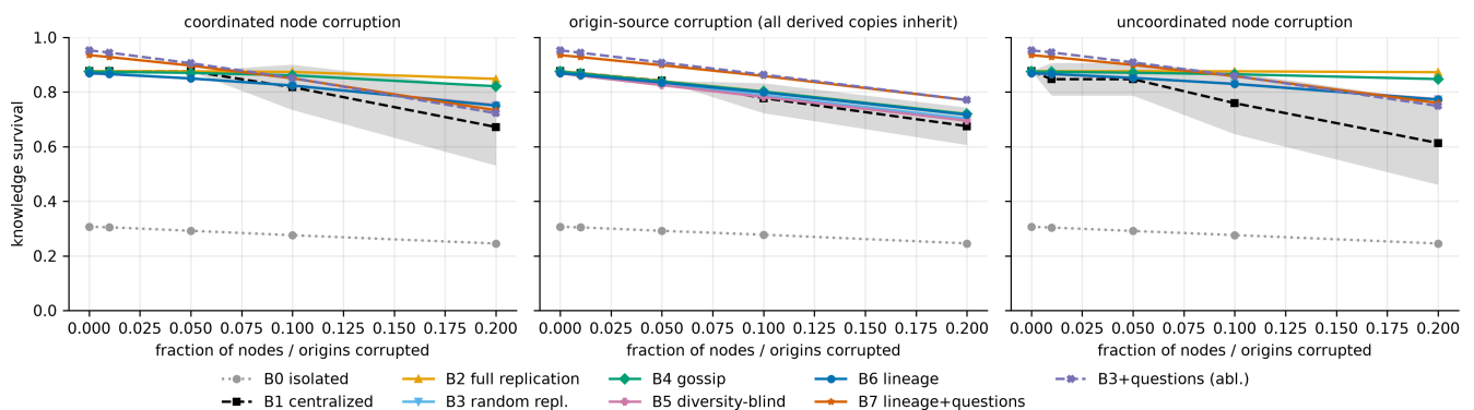
Misinformation resistance (N = 10,000, 30% random churn, 30 seeds, 95% CI)
