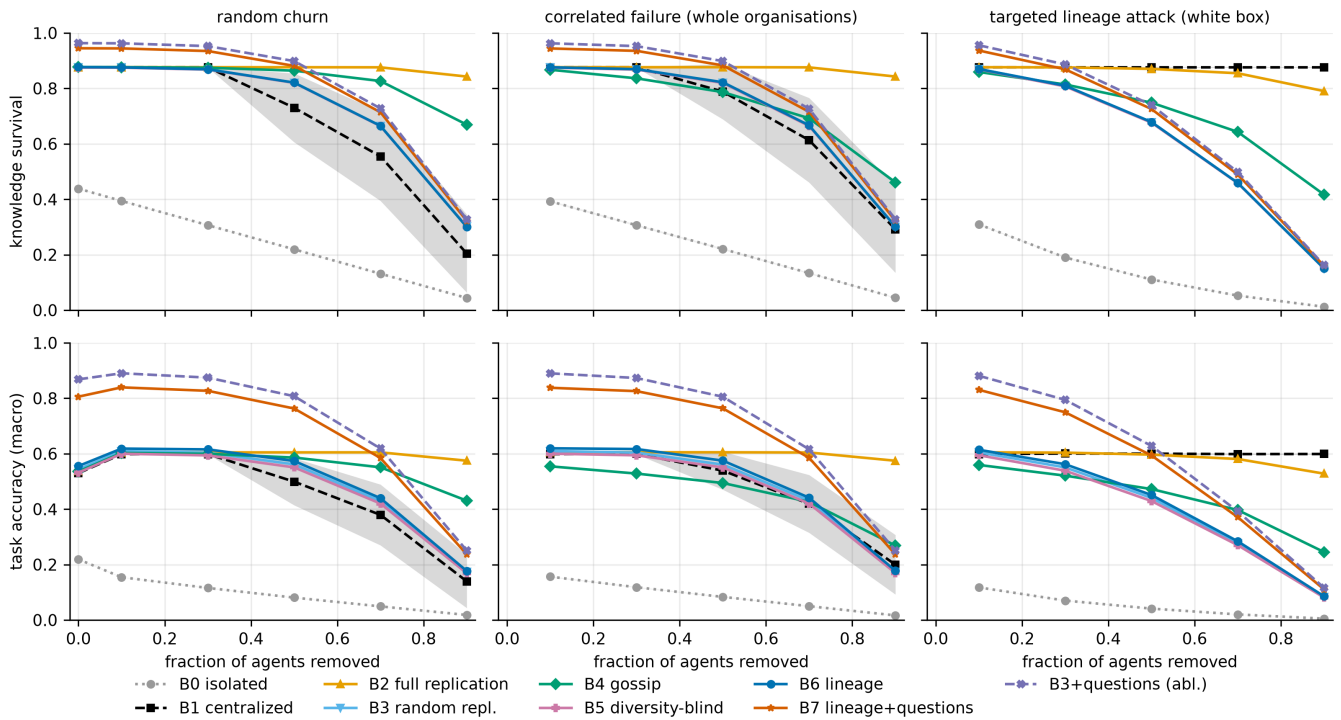
Knowledge survival under escalating failure (N = 10,000 agents, 30 seeds, 95% CI)
