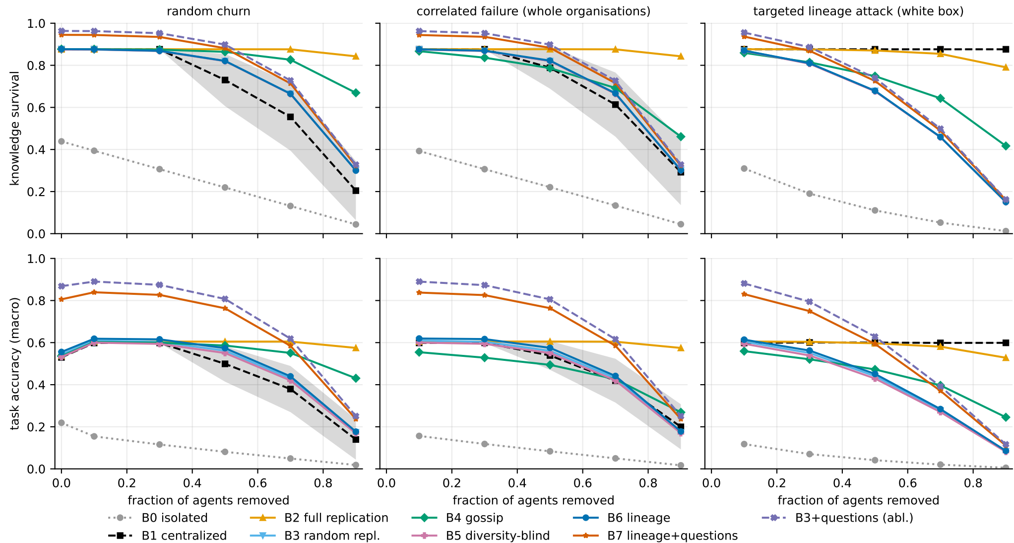
Knowledge survival under escalating failure (N = 10,000 agents, 30 seeds, 95% CI)
