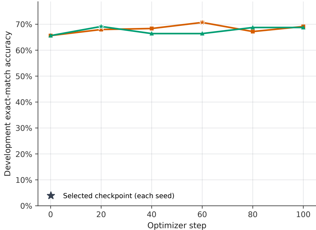
Development exact match · selected checkpoints
