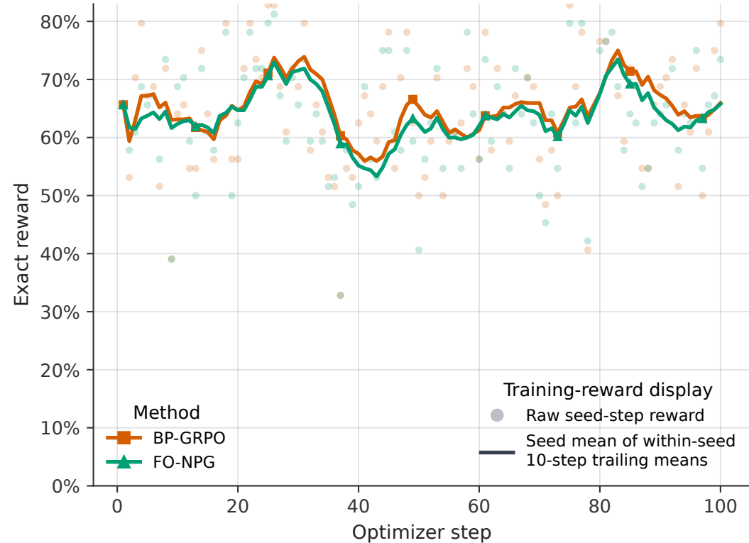
Training rollout exact reward
