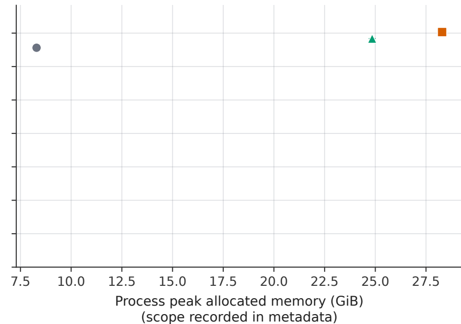
Memory footprint
