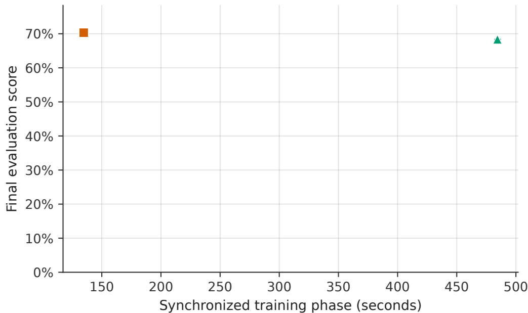
Optimizer efficiency
