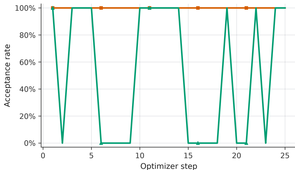
Update acceptance
