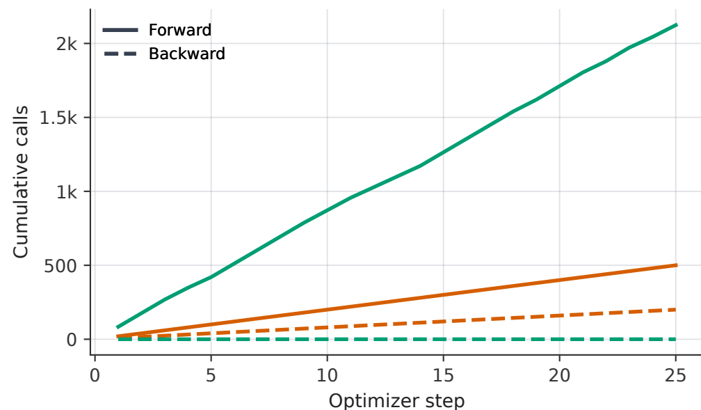
Model-call accounting
