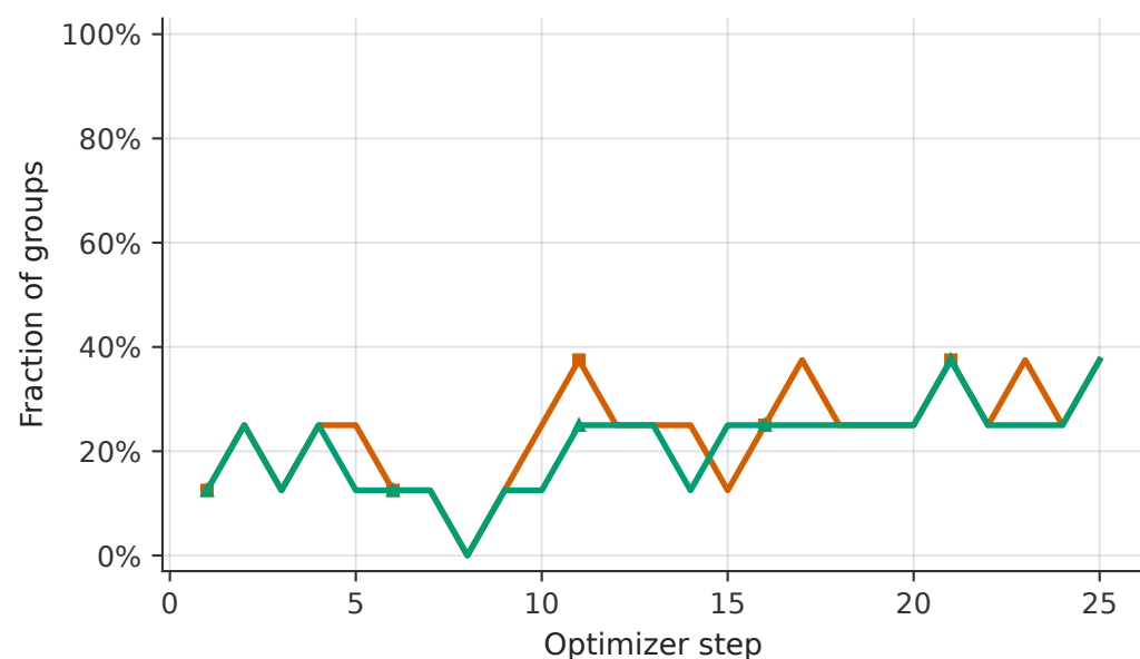
Model-call accounting
