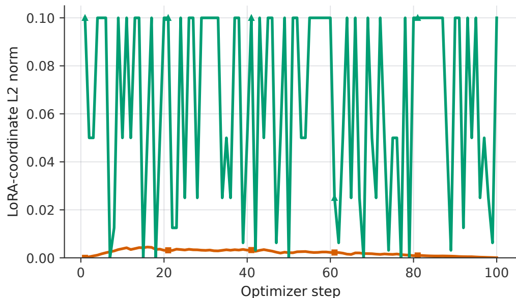
Applied policy-step norm
