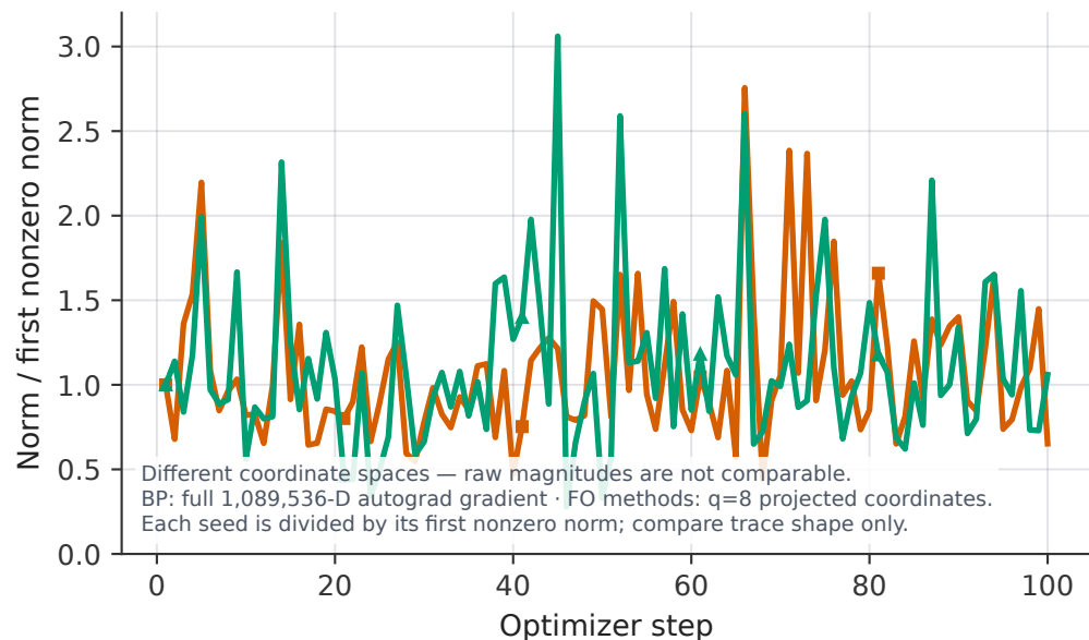
Applied policy-step norm
