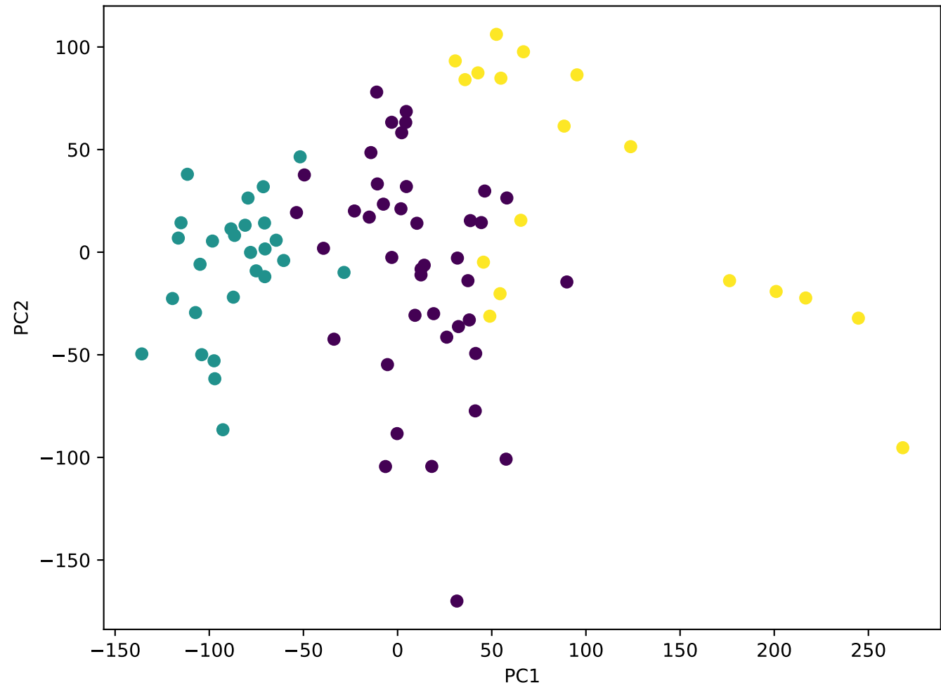
Agglomerative
