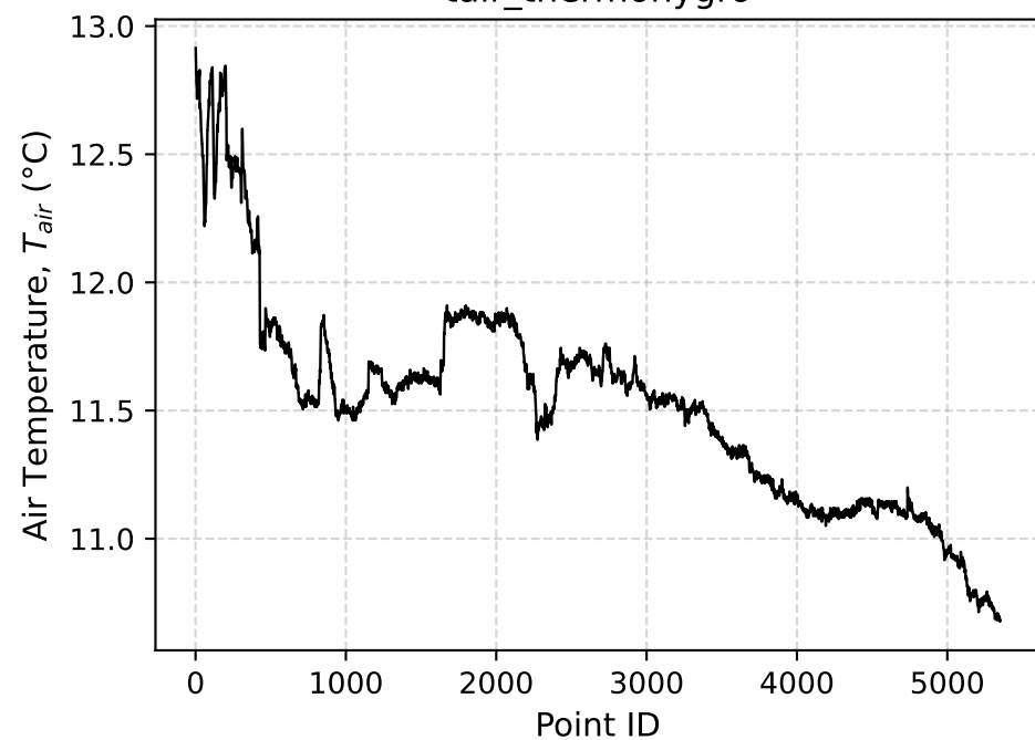
pet
