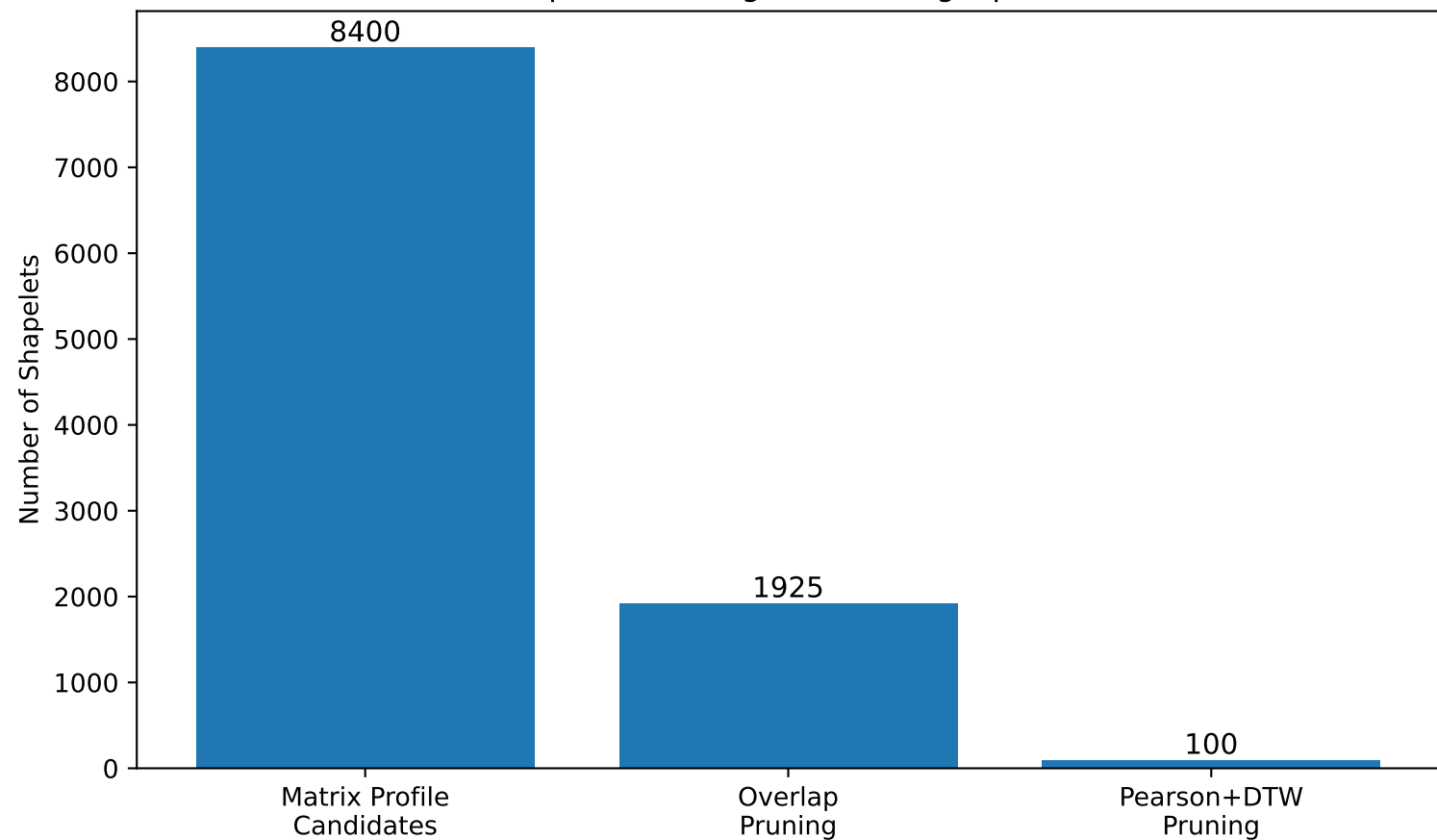
Shapelet Ranking and Pruning Pipeline
