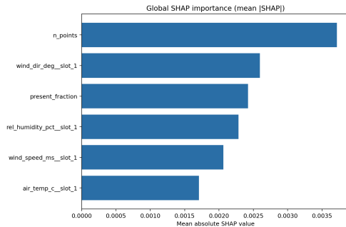
Global SHAP: top drivers.
