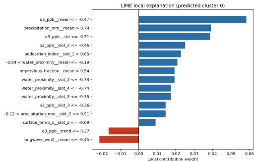
Local LIME explanation (example point).
