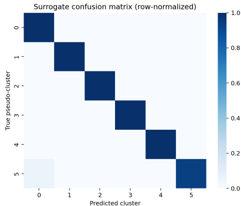
Surrogate confusion matrix.
