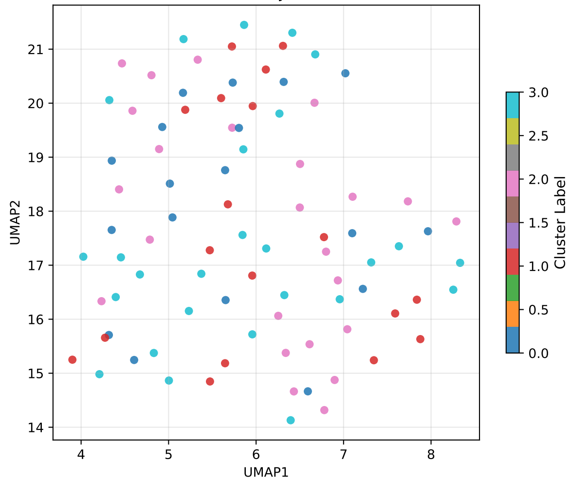
UMAP Projection
