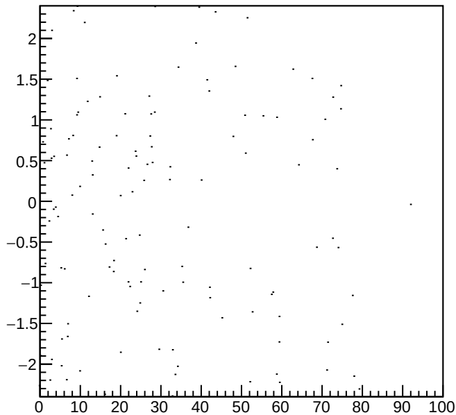
Electron#loose events
