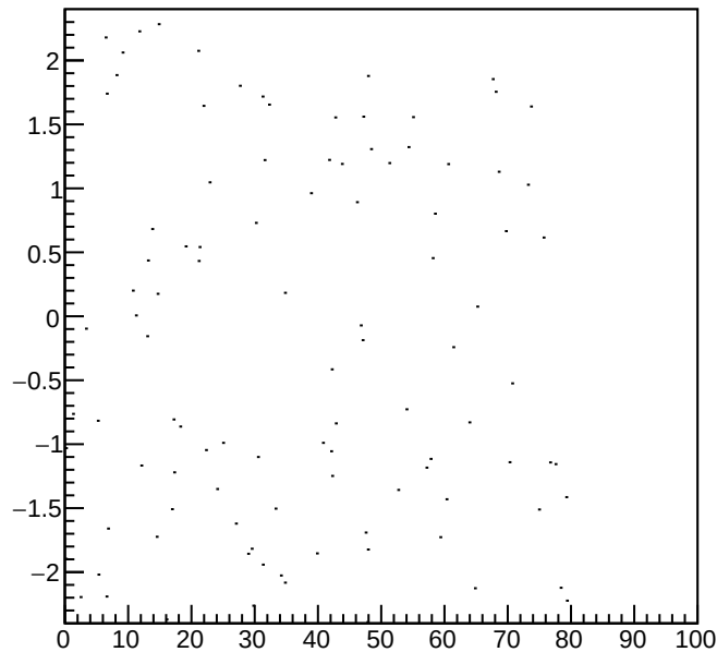
Electron#loose events
