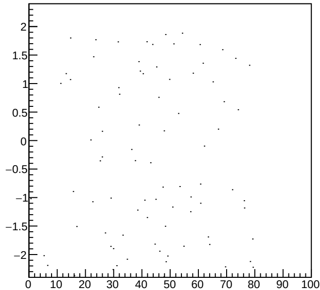
Electron#loose events_MC
