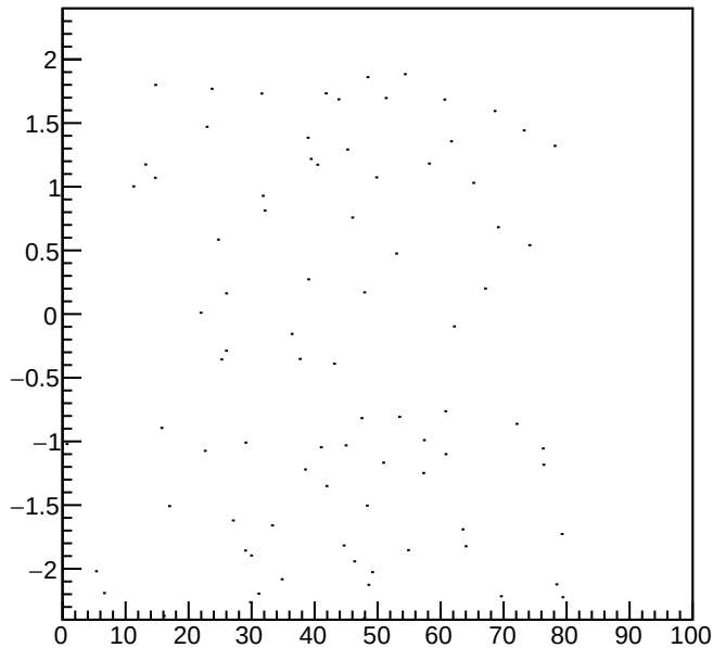
Electron#loose events_MC
