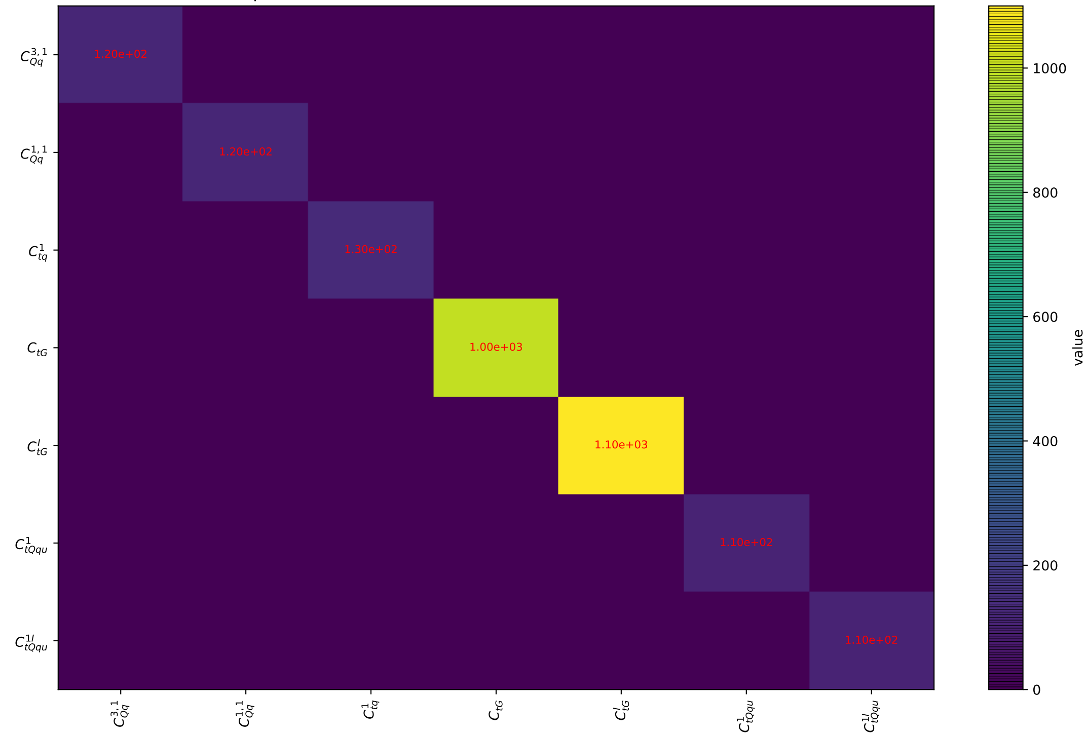
Quadratic dependence for tth from arXiv.1802.07237. Threshold: 1.0 (absolute value)
