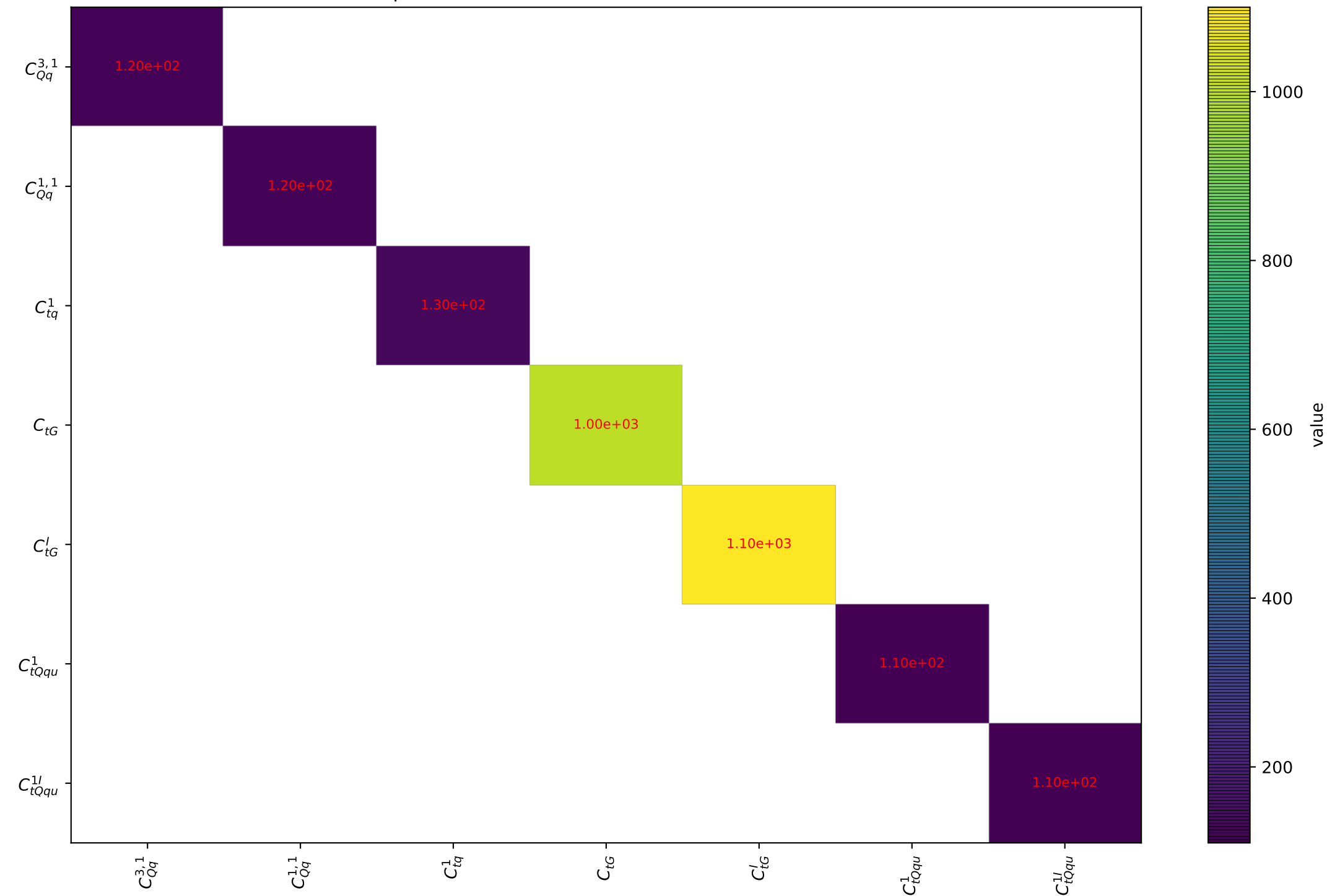
Quadratic dependence for tth from arXiv.1802.07237. Threshold: 0.1
