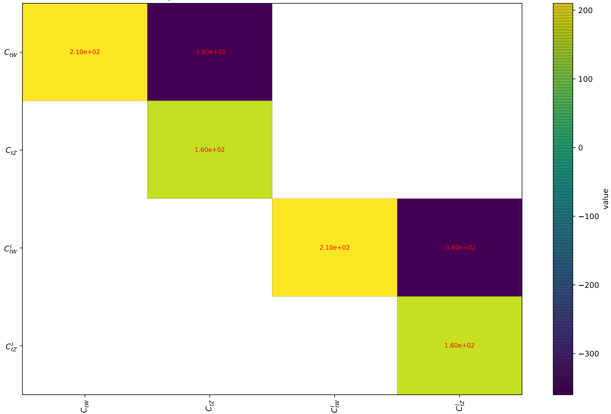
Quadratic dependence for tta from arXiv.1802.07237. Threshold: 100.0
