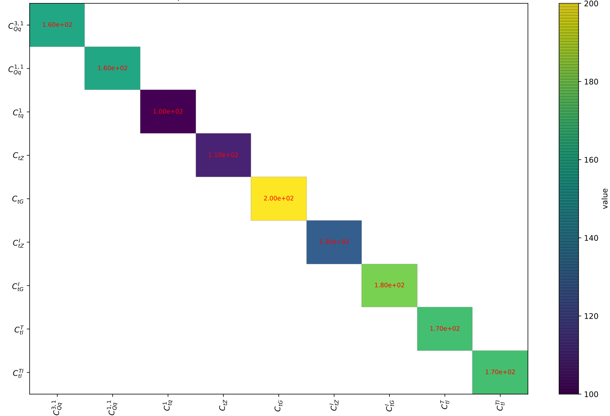
Quadratic dependence for ttee from arXiv.1802.07237. Threshold: 0.1
