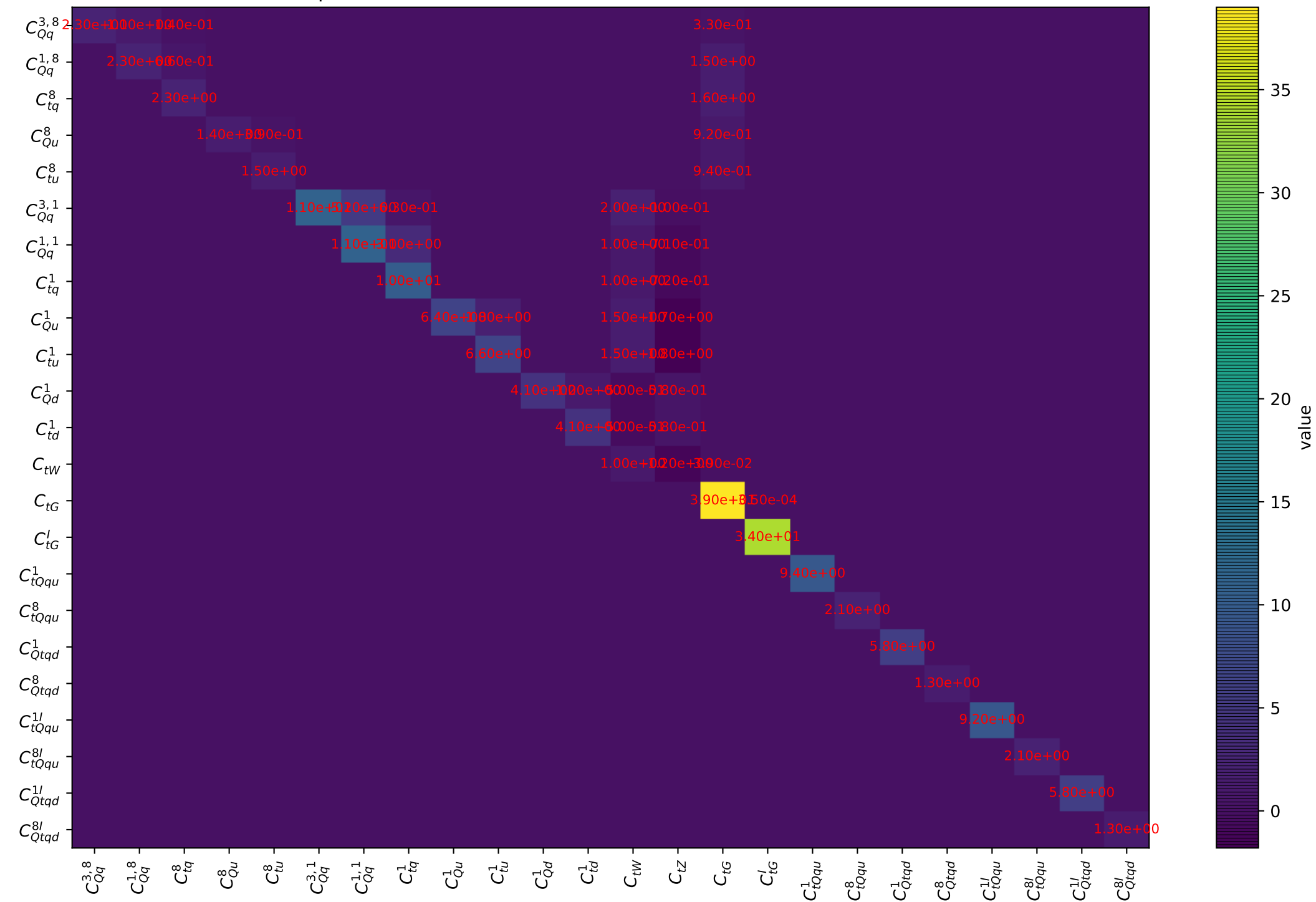
Quadratic dependence for tt from arXiv.1802.07237. Threshold: 1.0 (absolute value)
