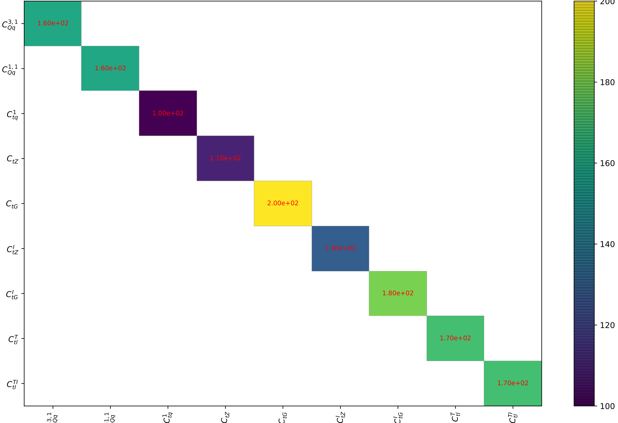
Quadratic dependence for ttee from arXiv.1802.07237. Threshold: 10.0
