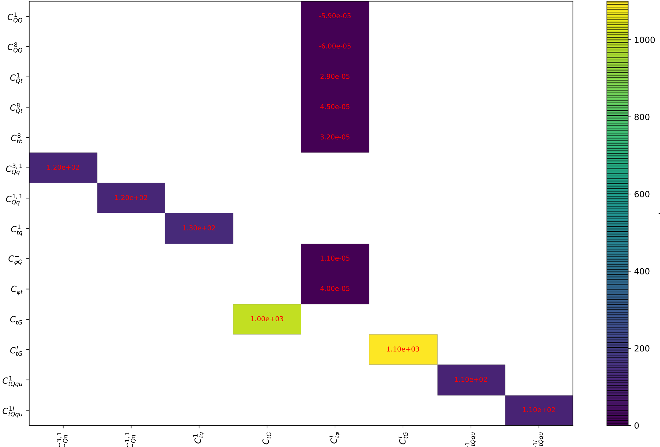
Quadratic dependence for tth from arXiv.1802.07237. Threshold: 0.0
