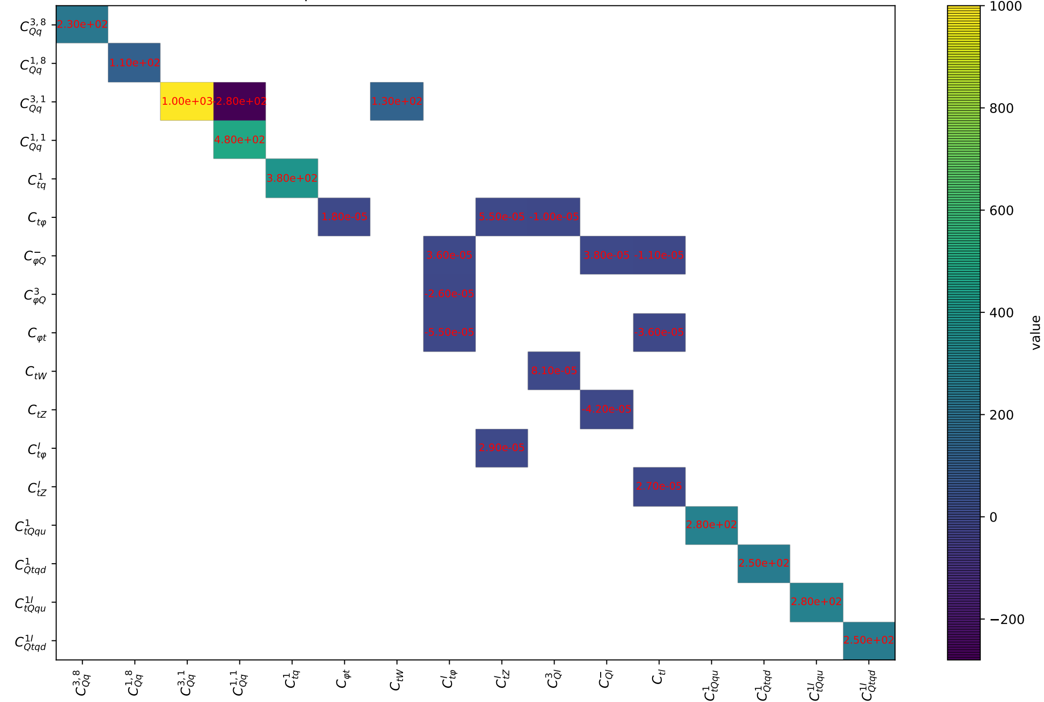
Quadratic dependence for ttev from arXiv.1802.07237. Threshold: 0.0
