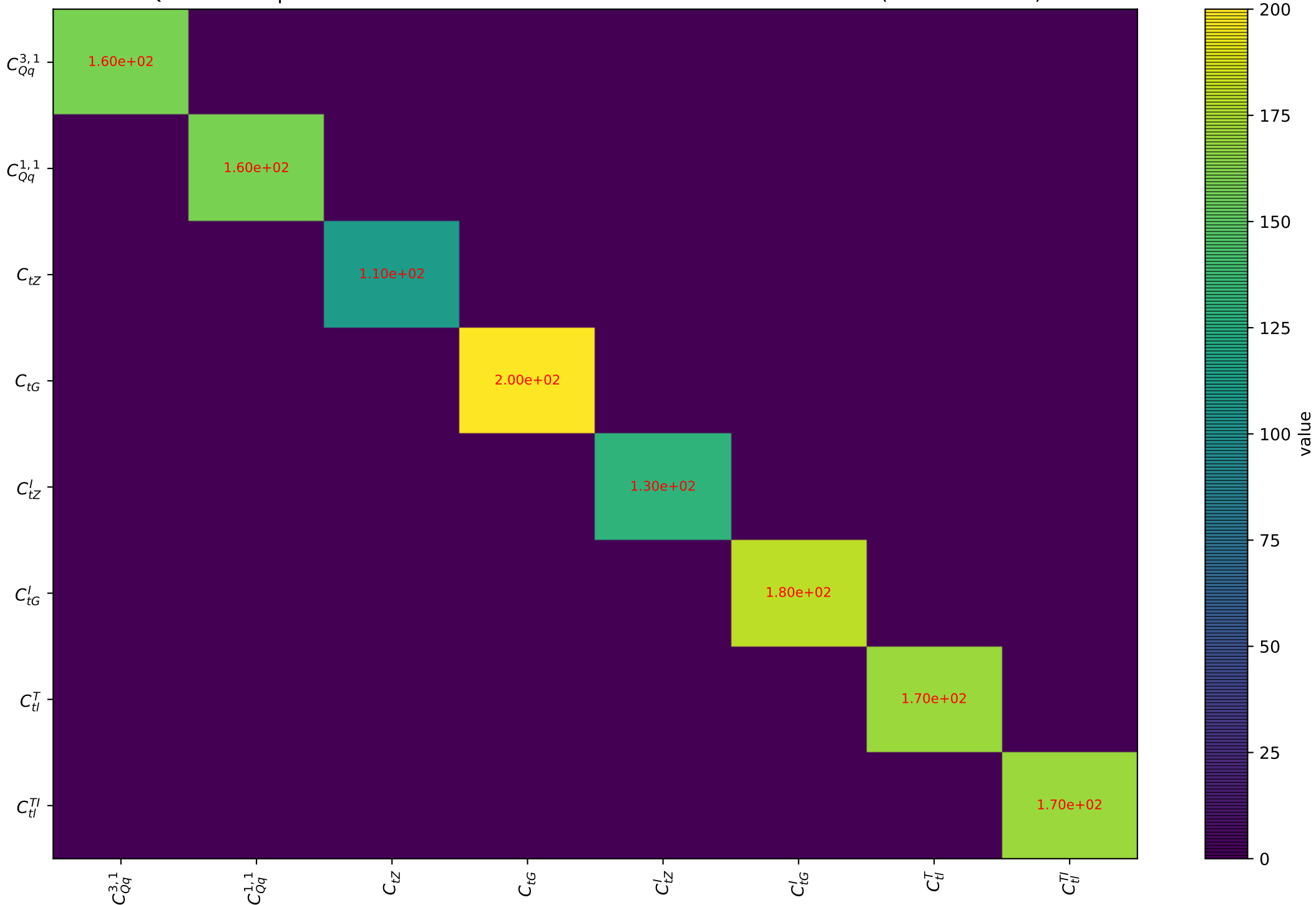
Quadratic dependence for ttee from arXiv.1802.07237. Threshold: 100.0 (absolute value)
