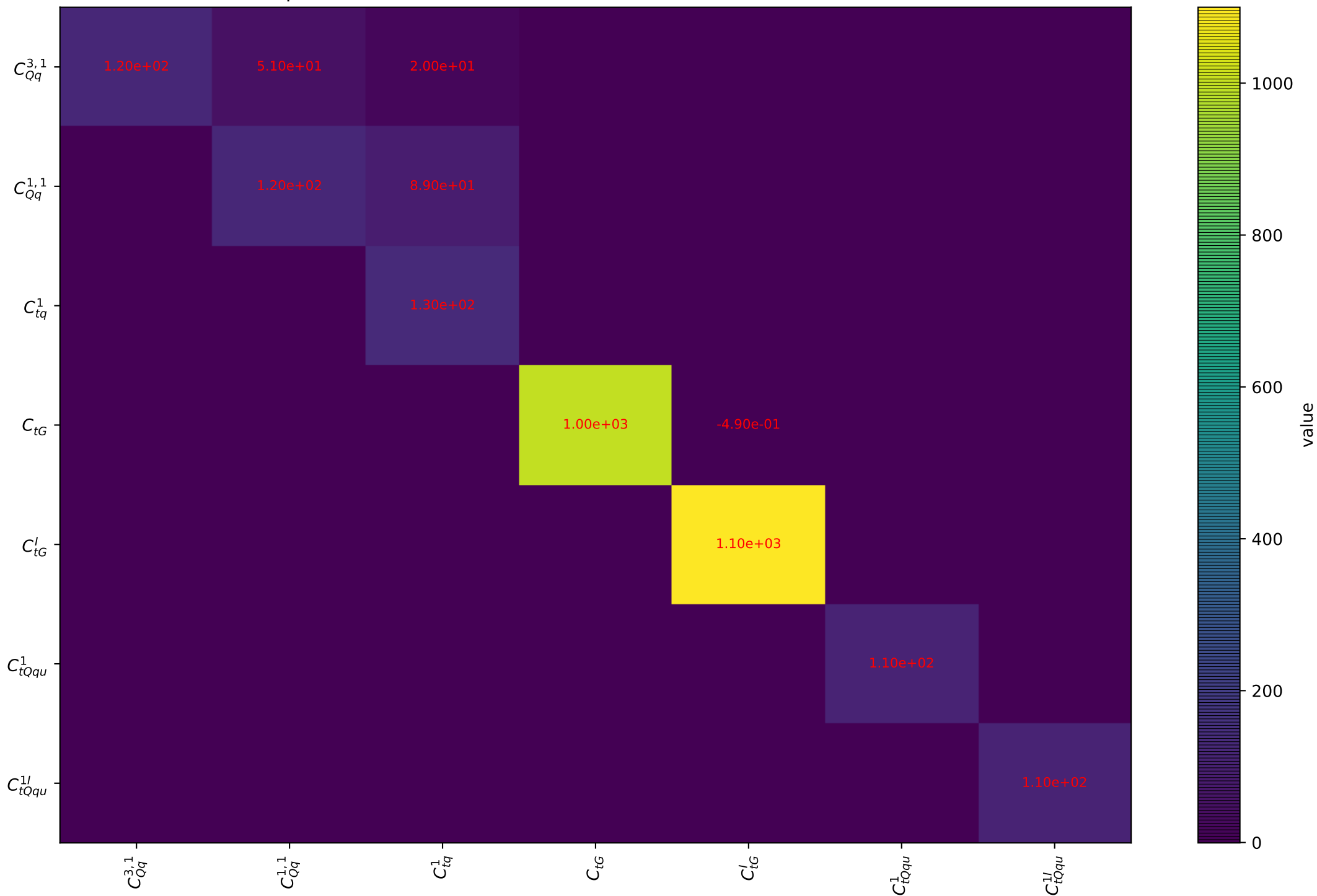
Quadratic dependence for tth from arXiv.1802.07237. Threshold: 100.0 (absolute value)
