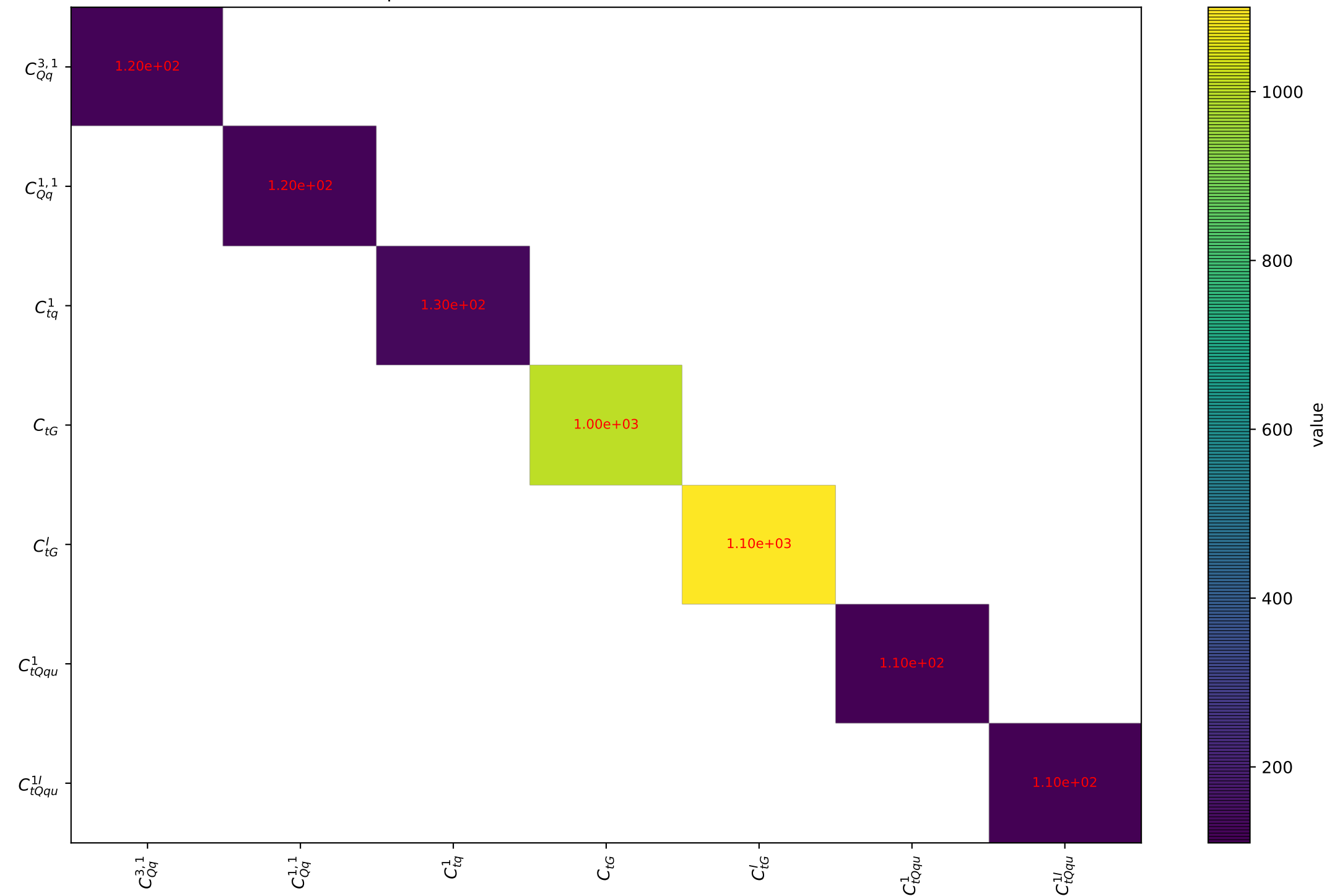
Quadratic dependence for tth from arXiv.1802.07237. Threshold: 10.0
