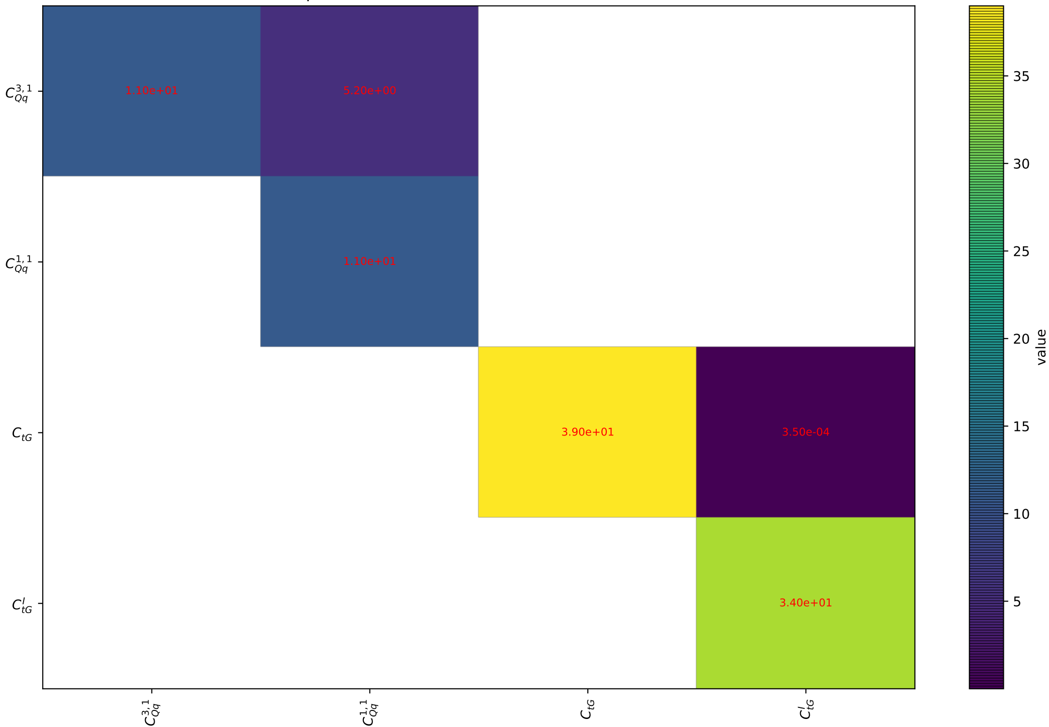
Quadratic dependence for tt from arXiv.1802.07237. Threshold: 10.0
