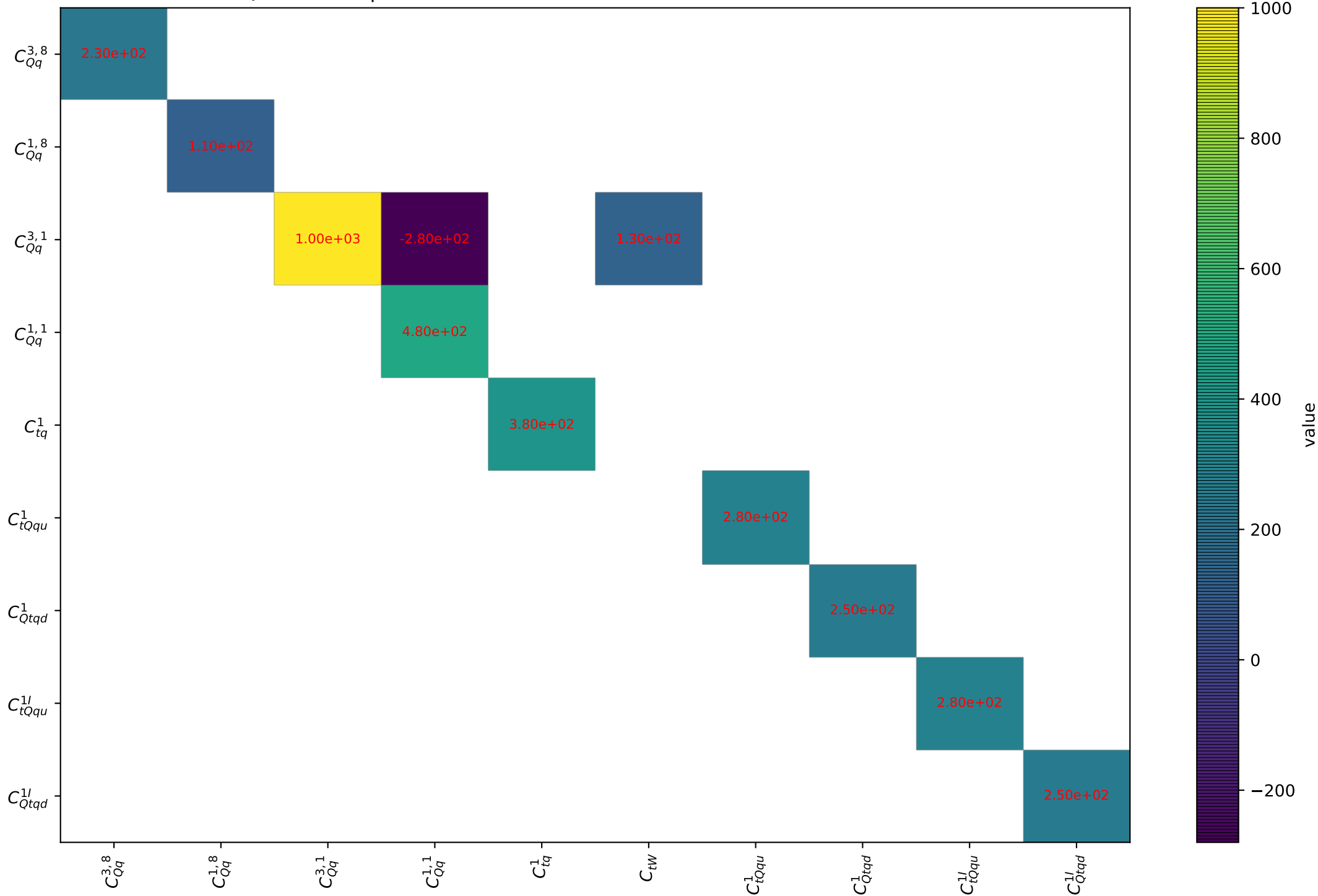
Quadratic dependence for ttev from arXiv.1802.07237. Threshold: 10.0
