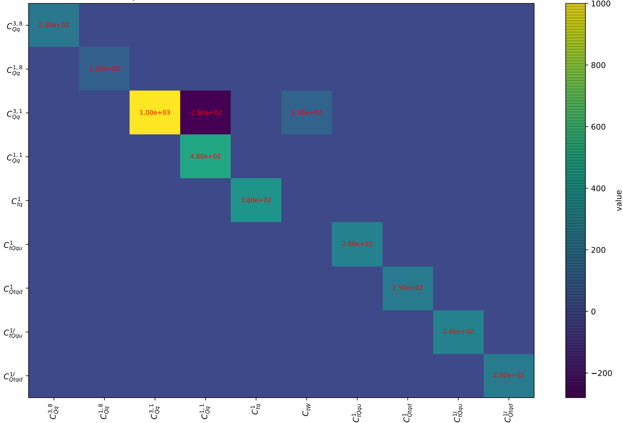
Quadratic dependence for ttev from arXiv.1802.07237. Threshold: 100.0 (absolute value)
