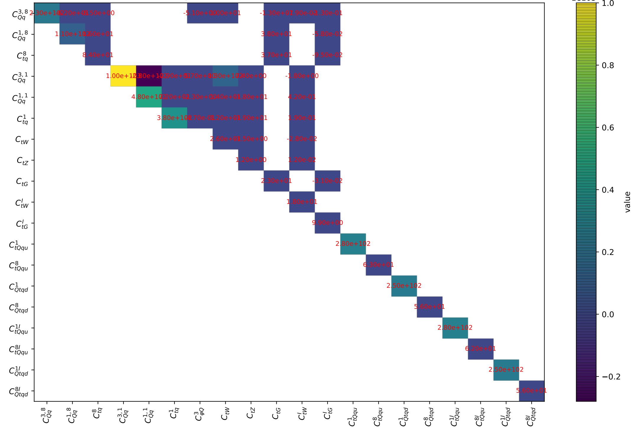
Quadratic dependence for ttev from arXiv.1802.07237. Threshold: 1.0
