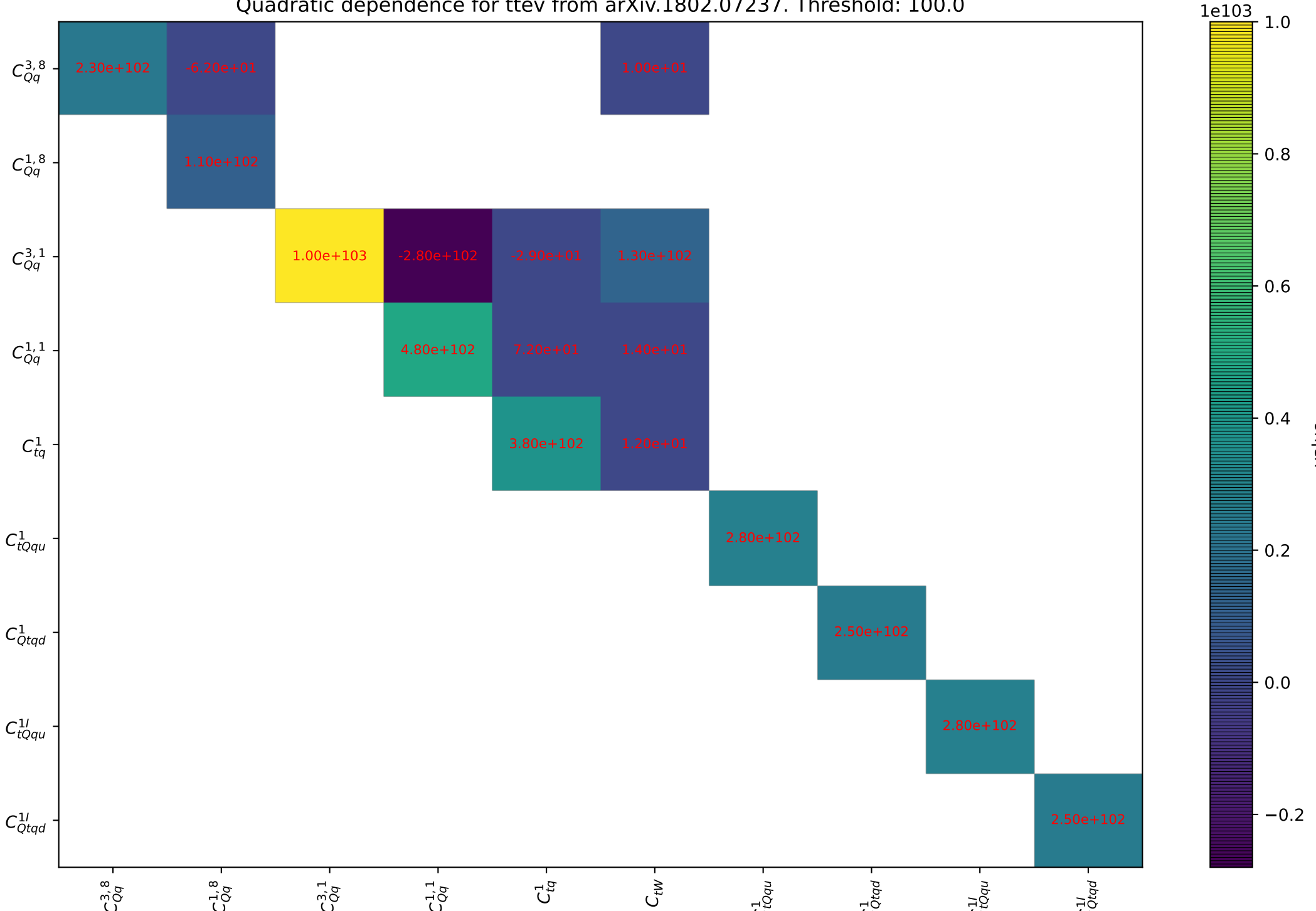
Quadratic dependence for ttev from arXiv.1802.07237. Threshold: 100.0
