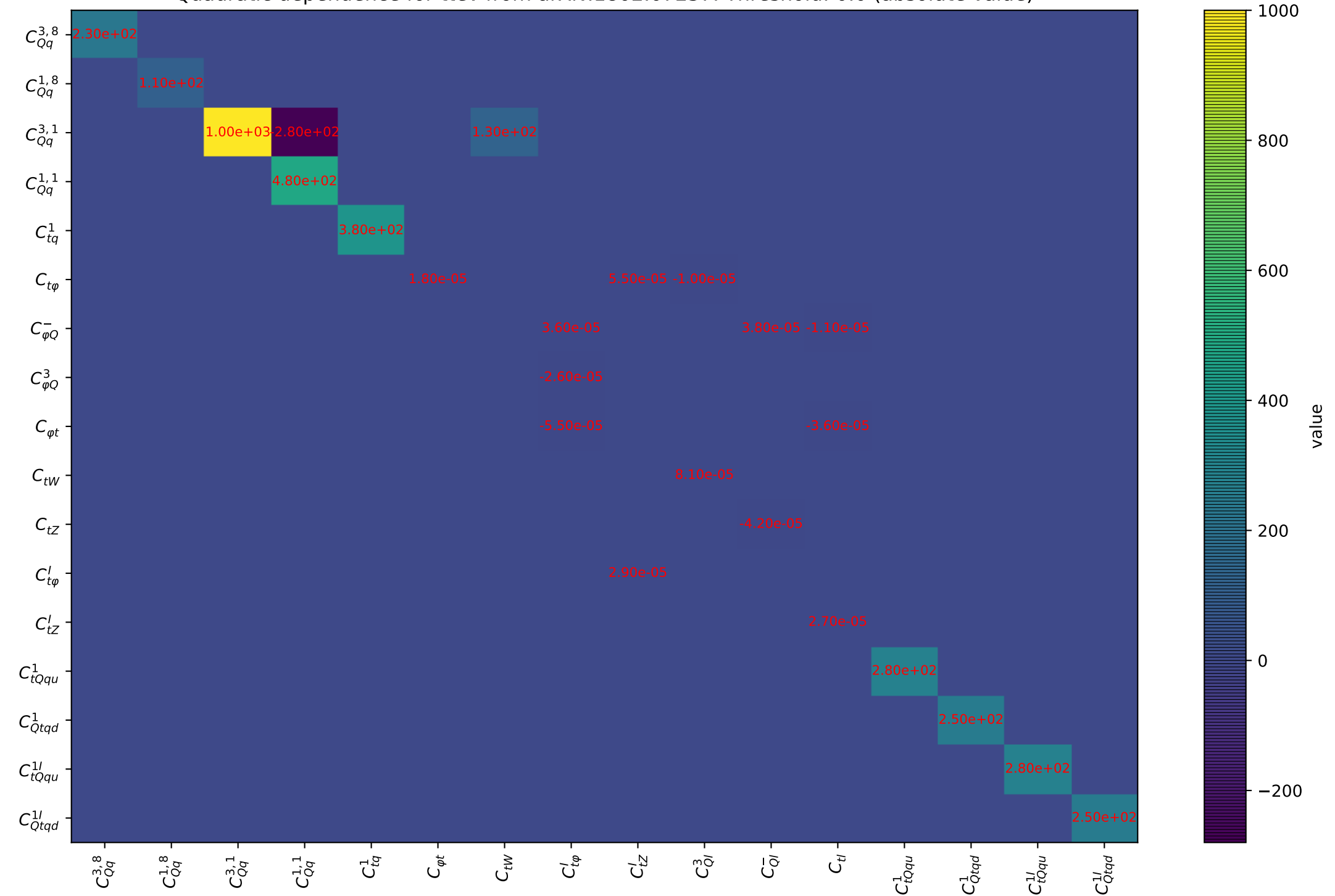
Quadratic dependence for ttev from arXiv.1802.07237. Threshold: 0.0 (absolute value)
