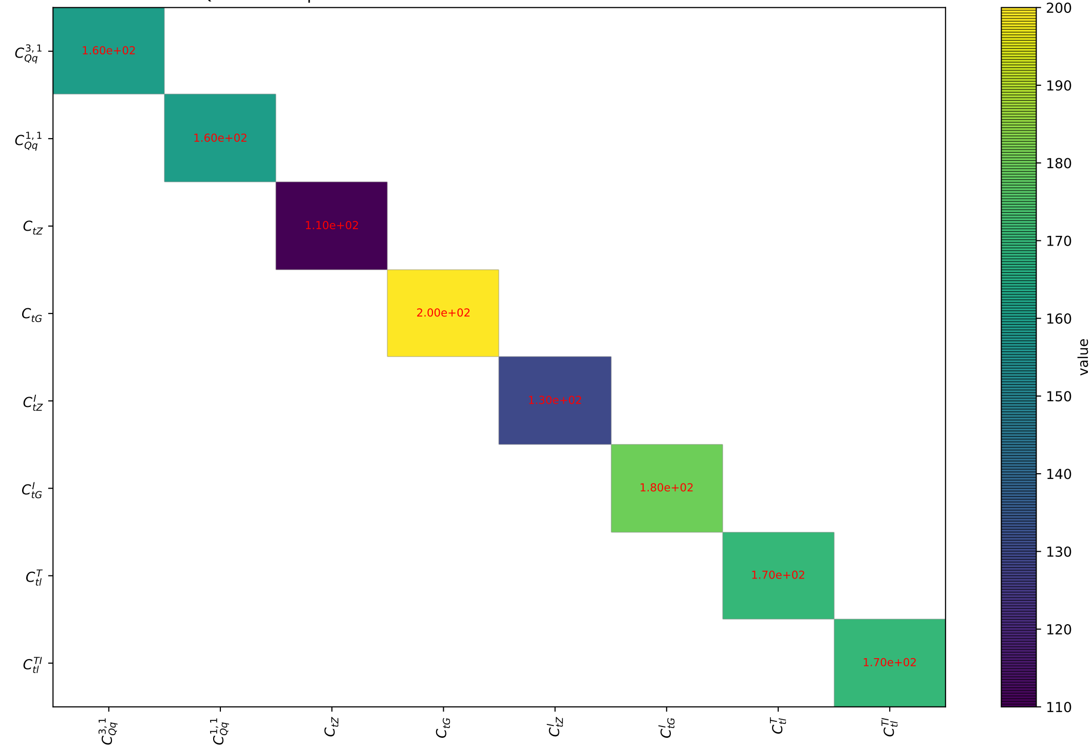
Quadratic dependence for ttee from arXiv.1802.07237. Threshold: 100.0
