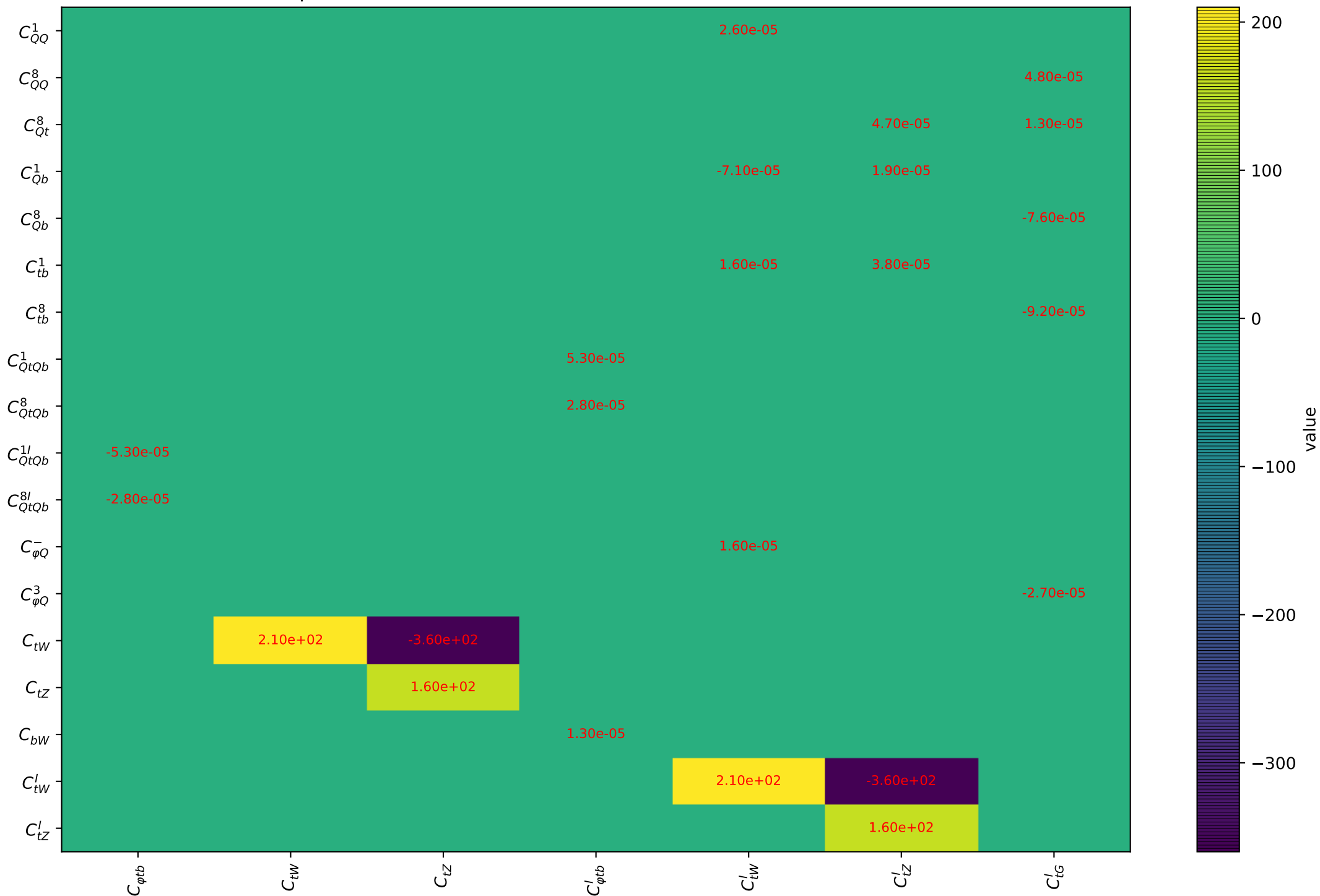
Quadratic dependence for tta from arXiv.1802.07237. Threshold: 0.0 (absolute value)
