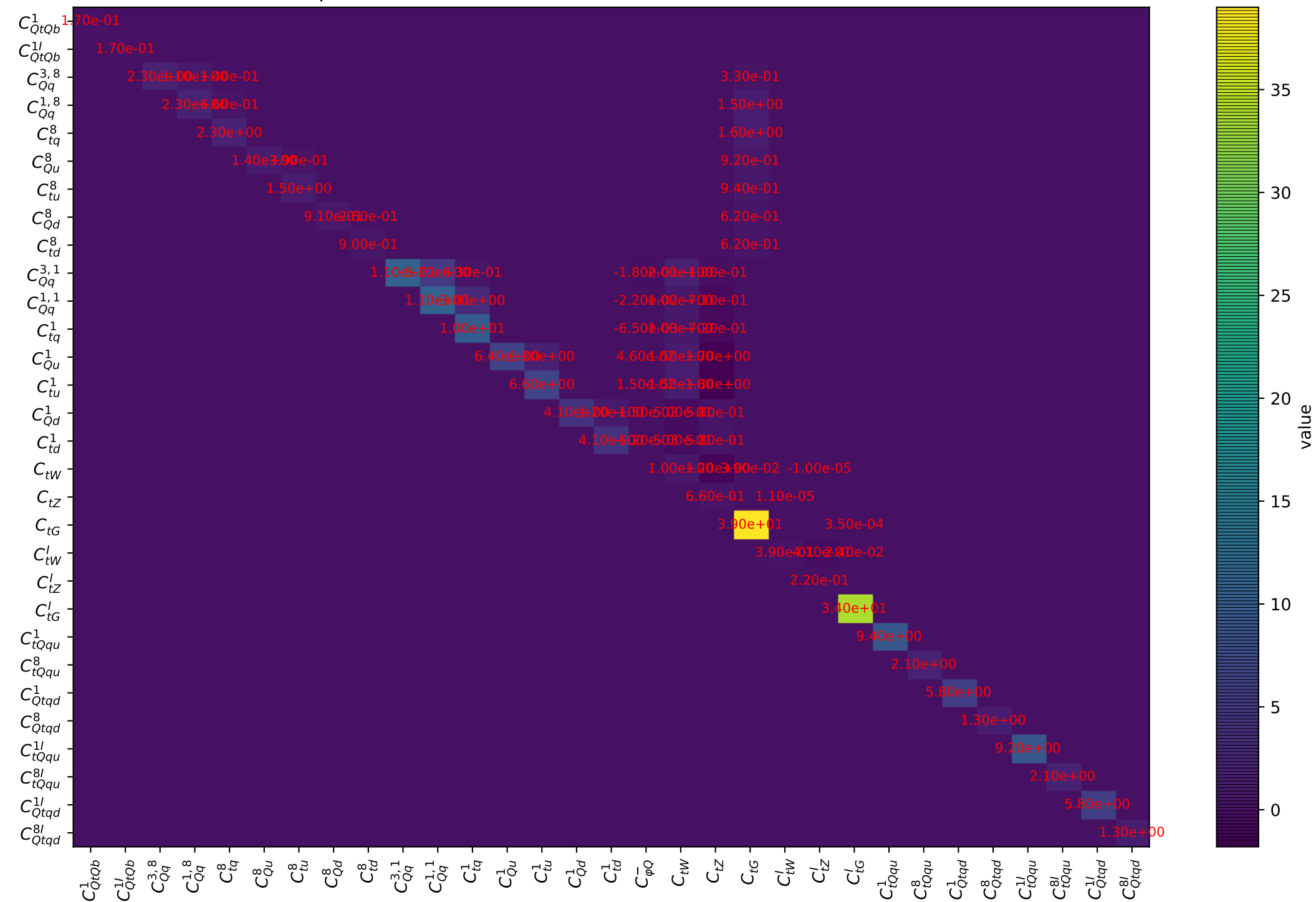
Quadratic dependence for tt from arXiv.1802.07237. Threshold: 0.1 (absolute value)
