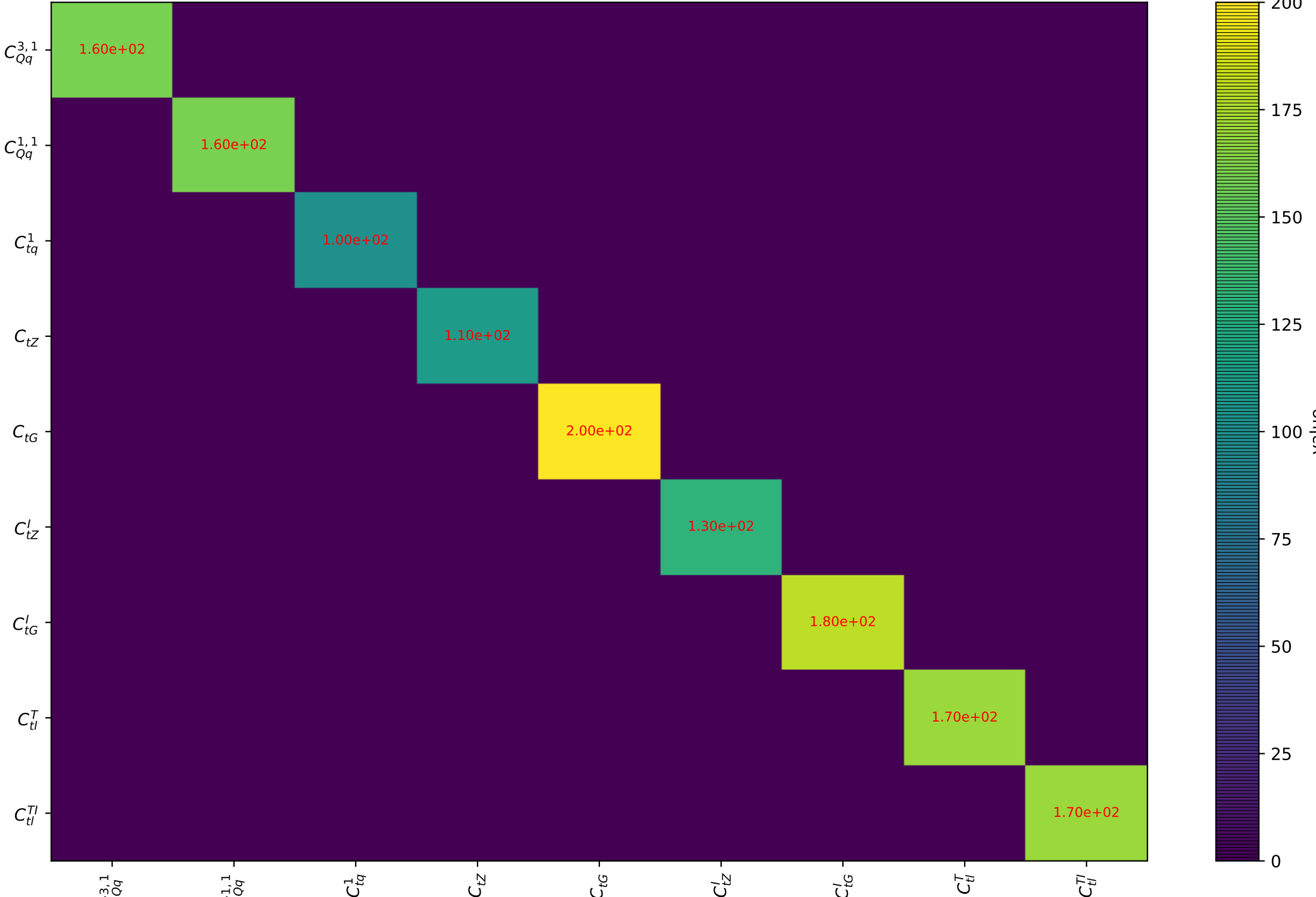
Quadratic dependence for ttee from arXiv.1802.07237. Threshold: 0.1 (absolute value)
