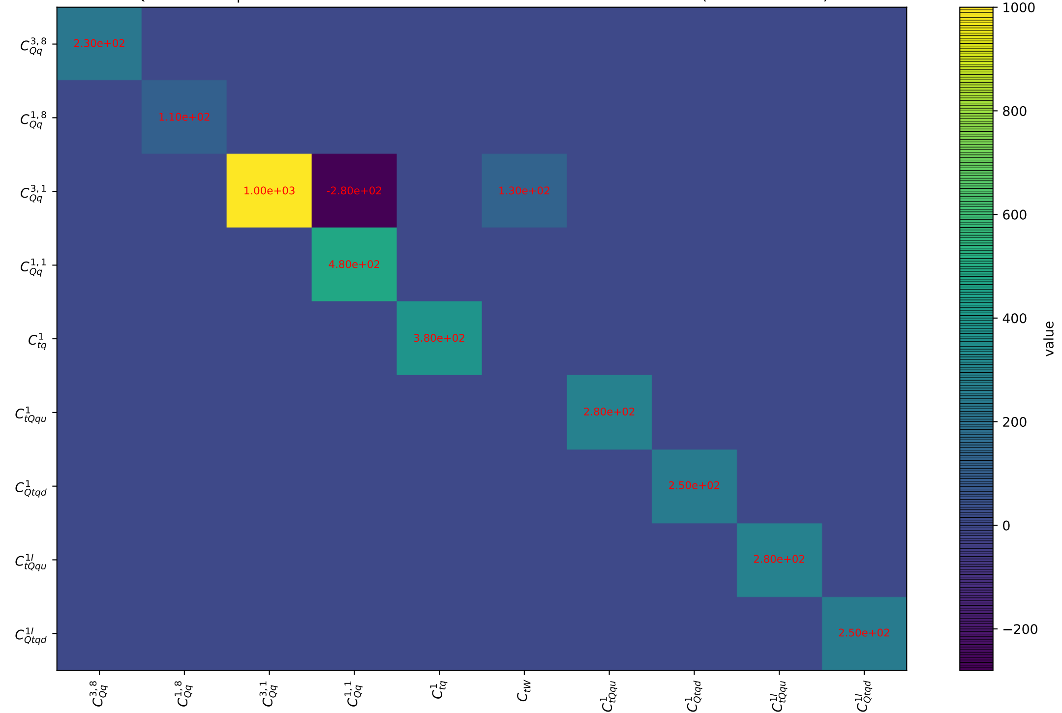
Quadratic dependence for ttev from arXiv.1802.07237. Threshold: 10.0 (absolute value)
