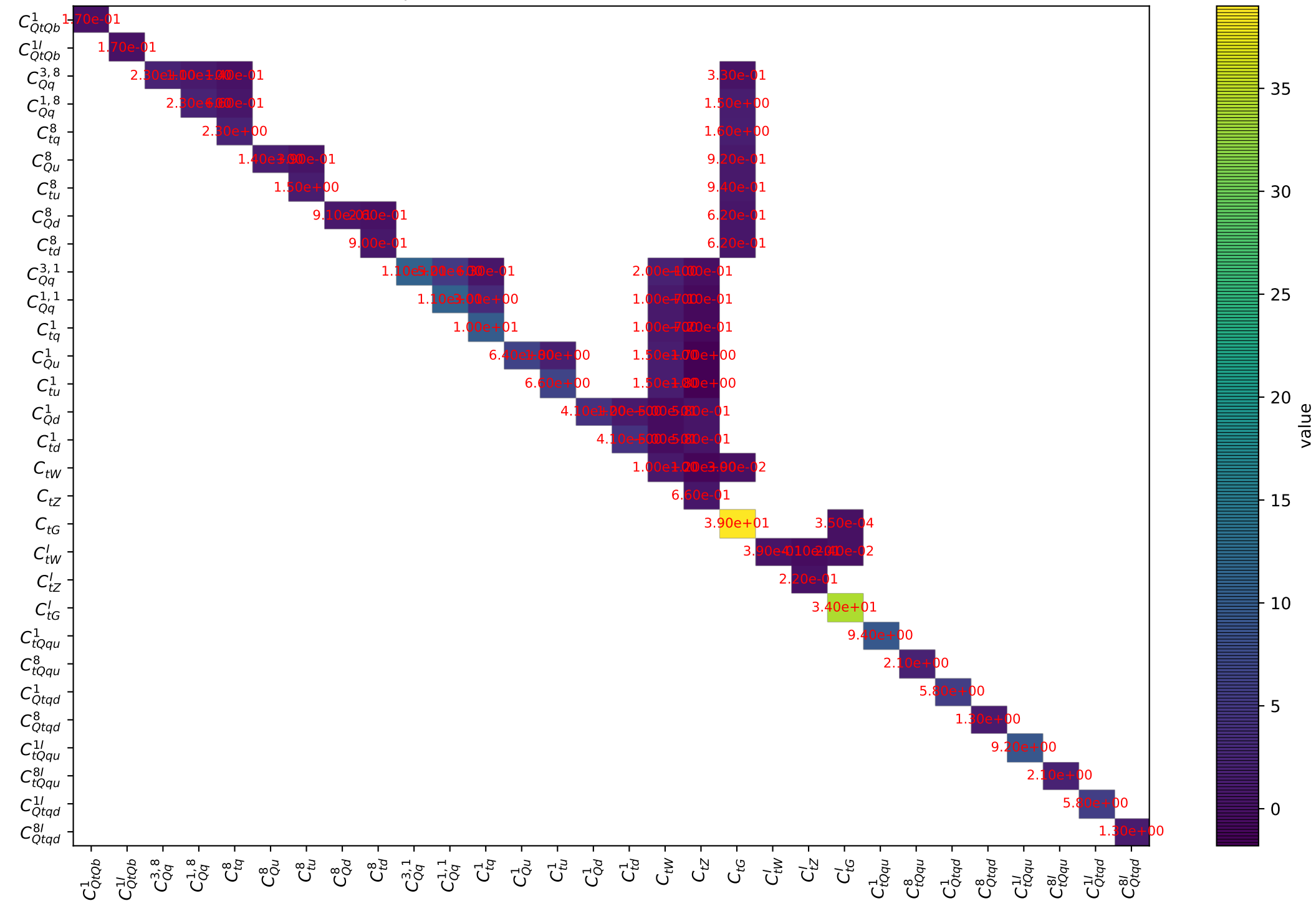
Quadratic dependence for tt from arXiv.1802.07237. Threshold: 0.1
