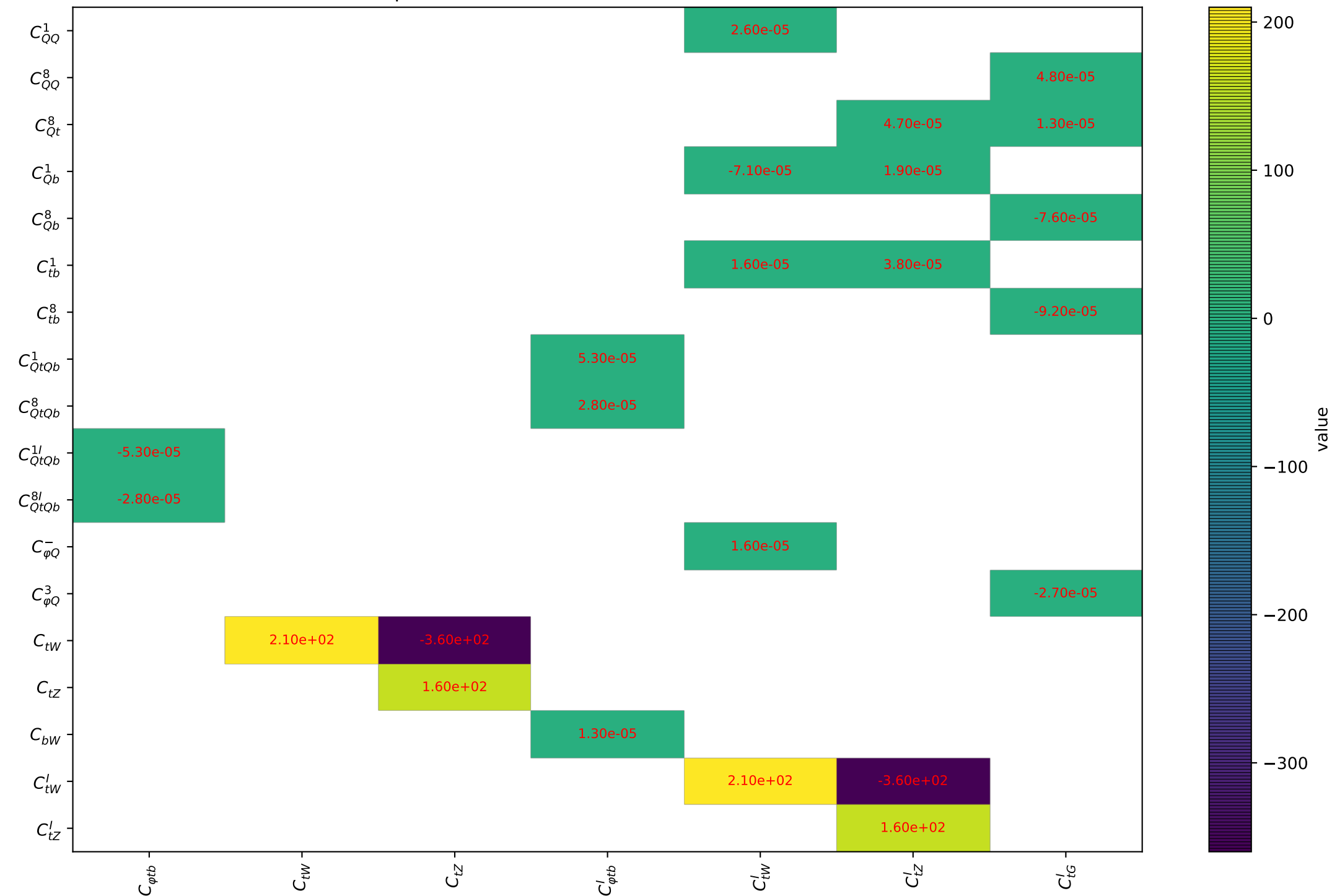
Quadratic dependence for tta from arXiv.1802.07237. Threshold: 0.0
