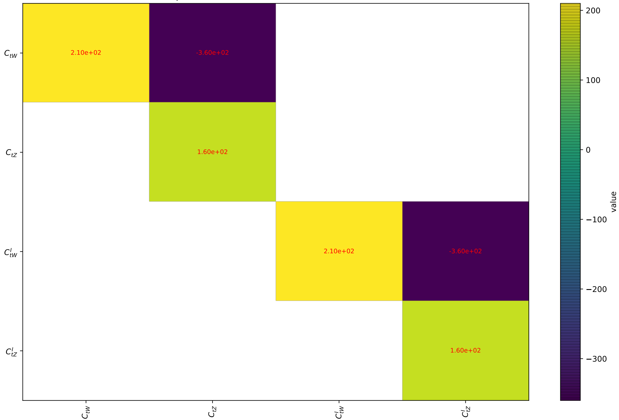
Quadratic dependence for tta from arXiv.1802.07237. Threshold: 0.1
