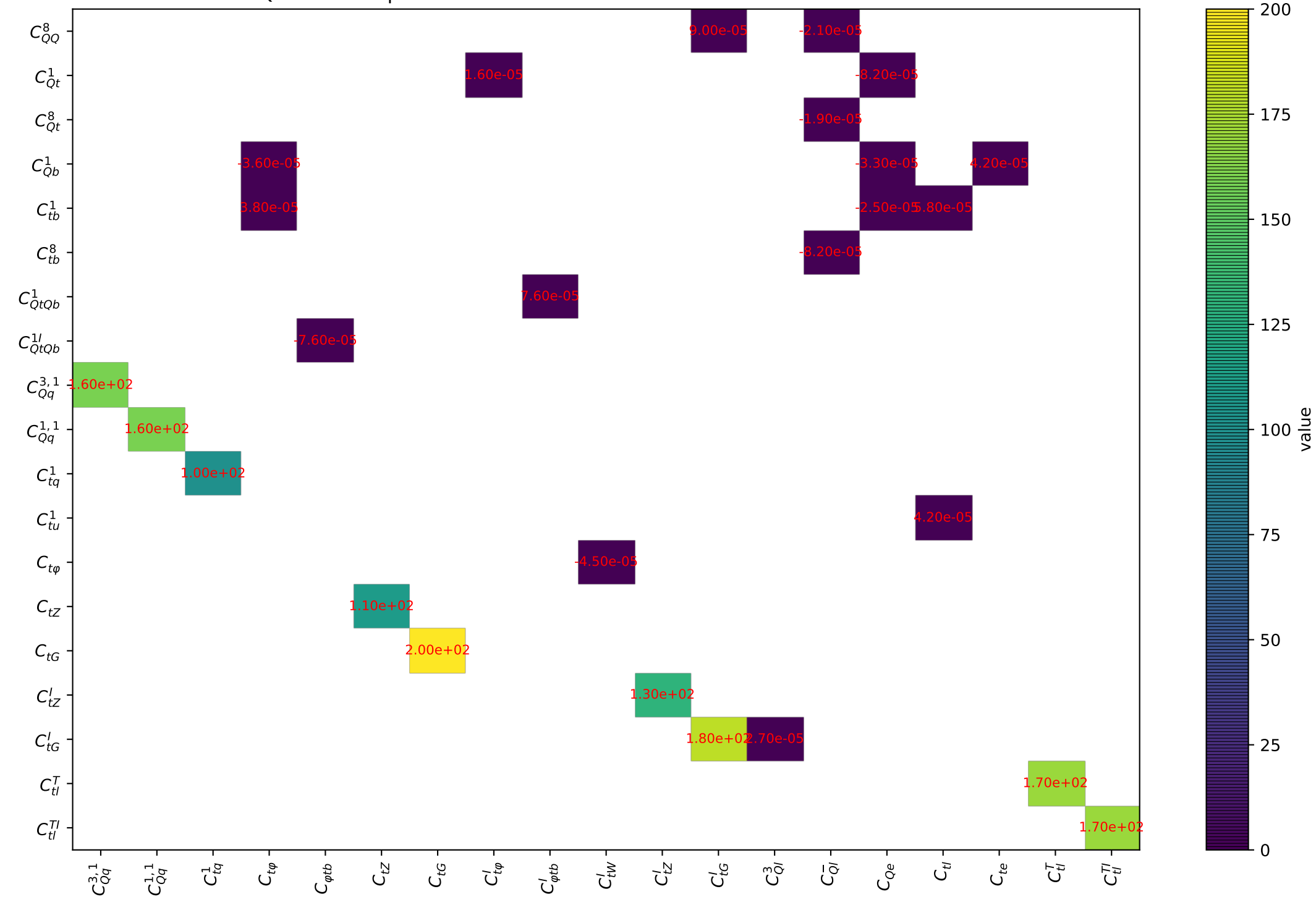
Quadratic dependence for ttee from arXiv.1802.07237. Threshold: 0.0
