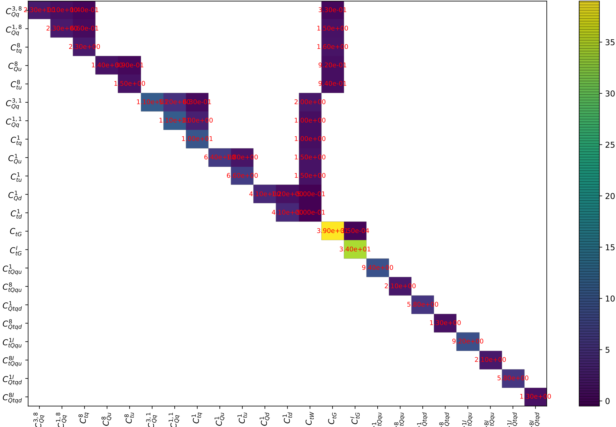
Quadratic dependence for tt from arXiv.1802.07237. Threshold: 1.0
