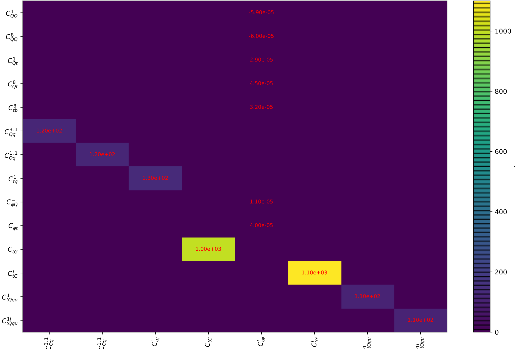
Quadratic dependence for tth from arXiv.1802.07237. Threshold: 0.0 (absolute value)
