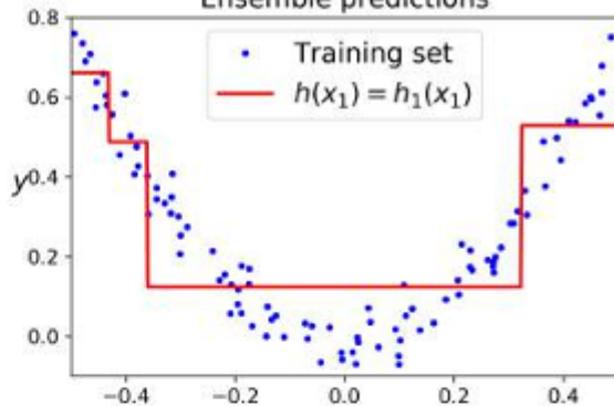
Ensemble predictions
