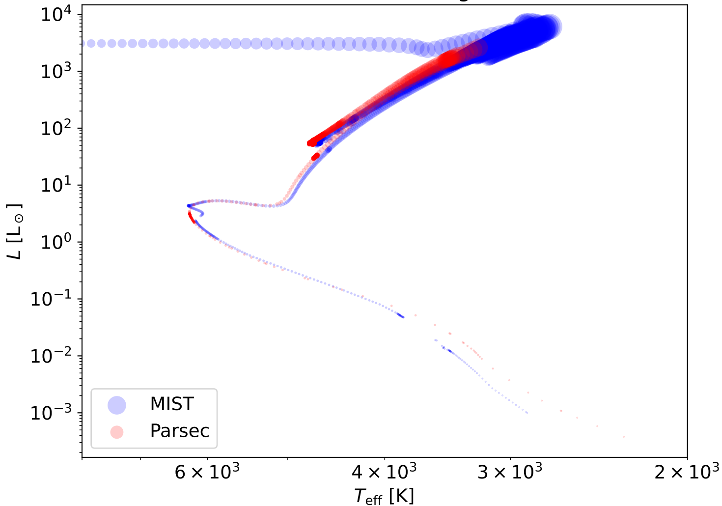
Isochrone at [\text{Fe}/\text{H}]=0.0 , age = 4.47 Ga
