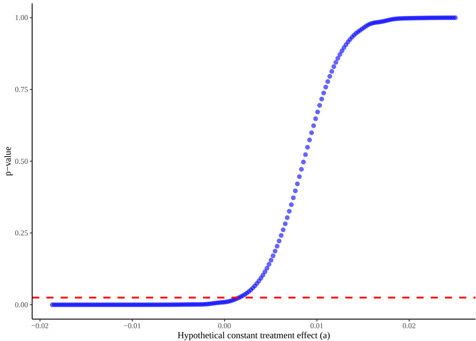
P-values across different hypothetical constant treatment effect for cg03995486
