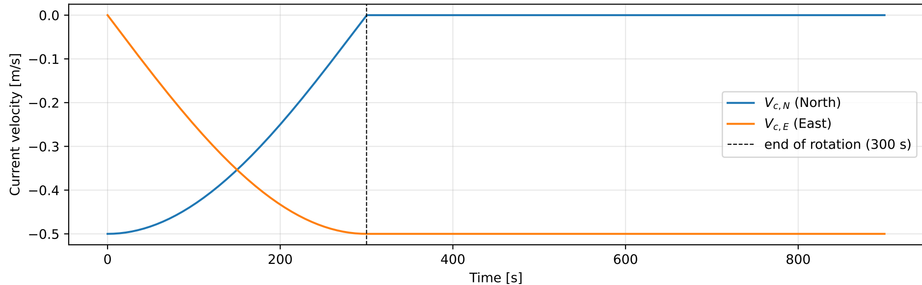
Simulation 2: NED current components
