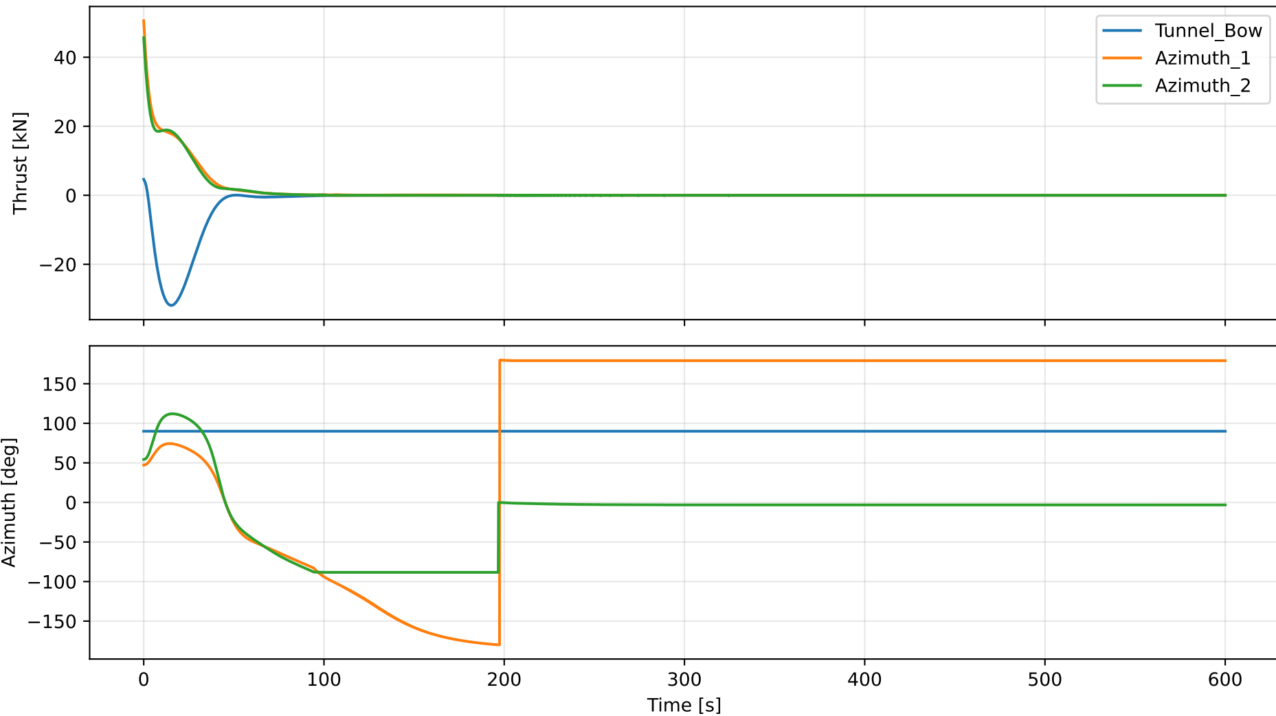
Thrusters
