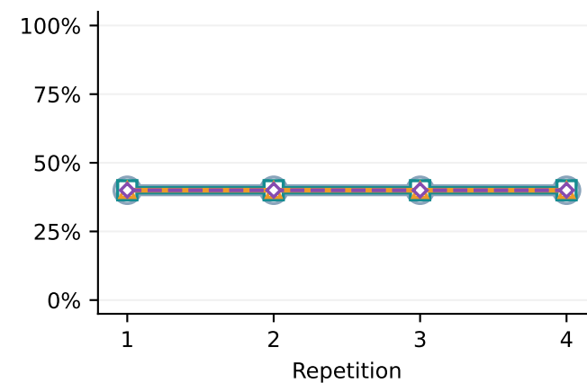
GLM 5.3
