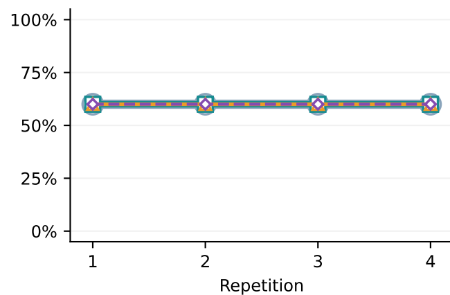
Qwen 3.8 27B
