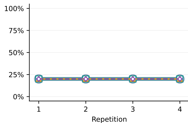
Claude Haiku 4.5
