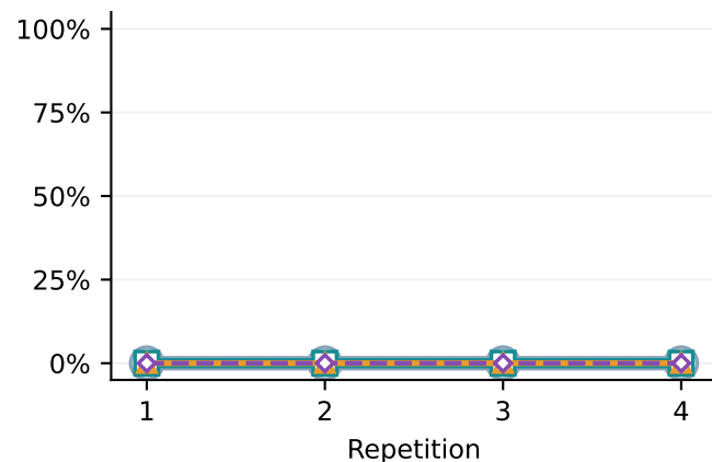
Qwen 3.8 27B
