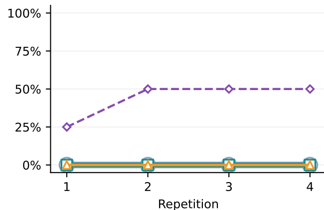
Claude Haiku 4.5
