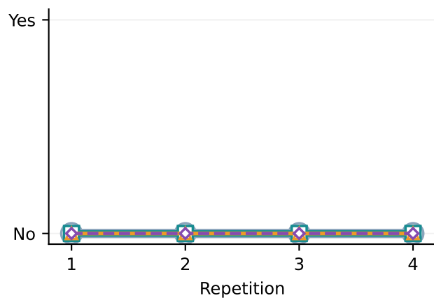
Qwen 3.8 27B
