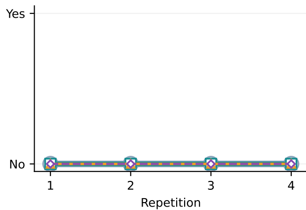
Claude Haiku 4.5
