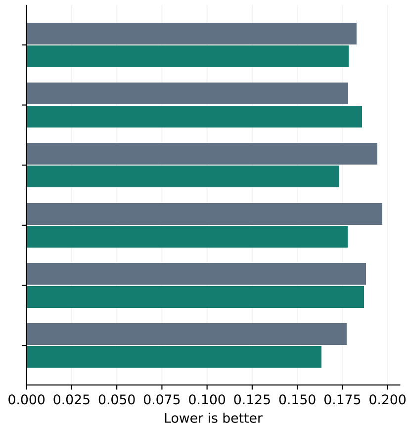
Native-score MSE
