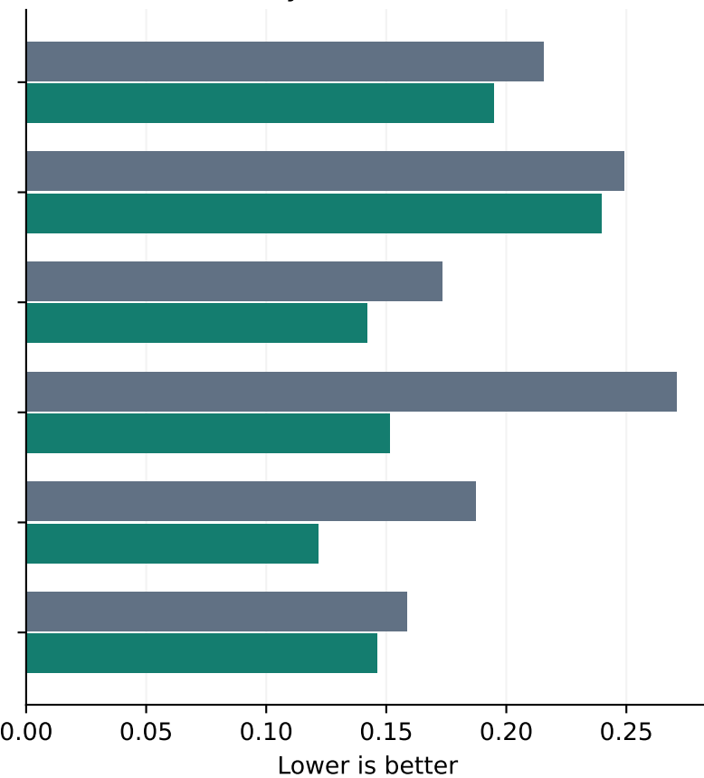
Any-invalid Brier
