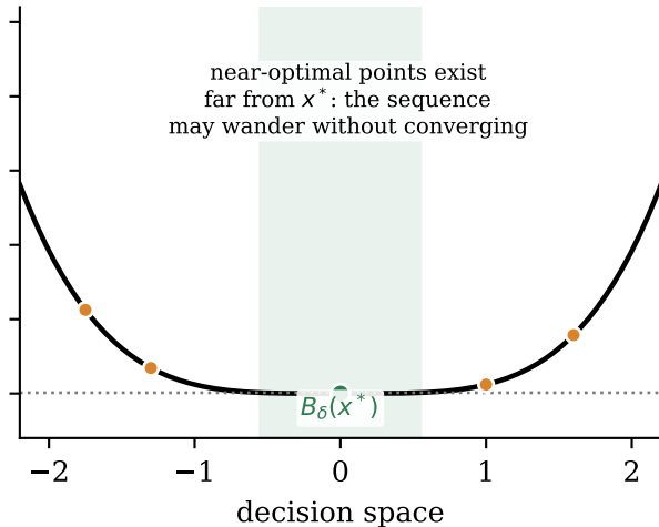
(b) Shallow valley: condition fails
