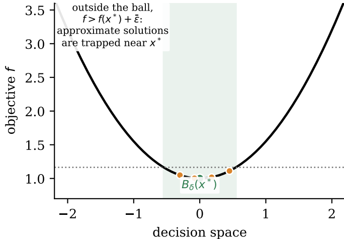
(a) Sharp minimum: condition holds
