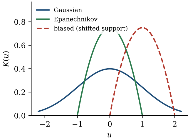
(a) Kernel functions
