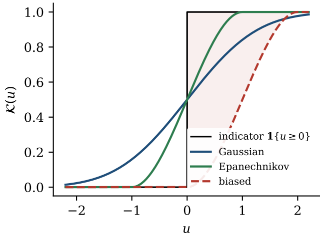
(b) Integrated kernels vs the indicator
