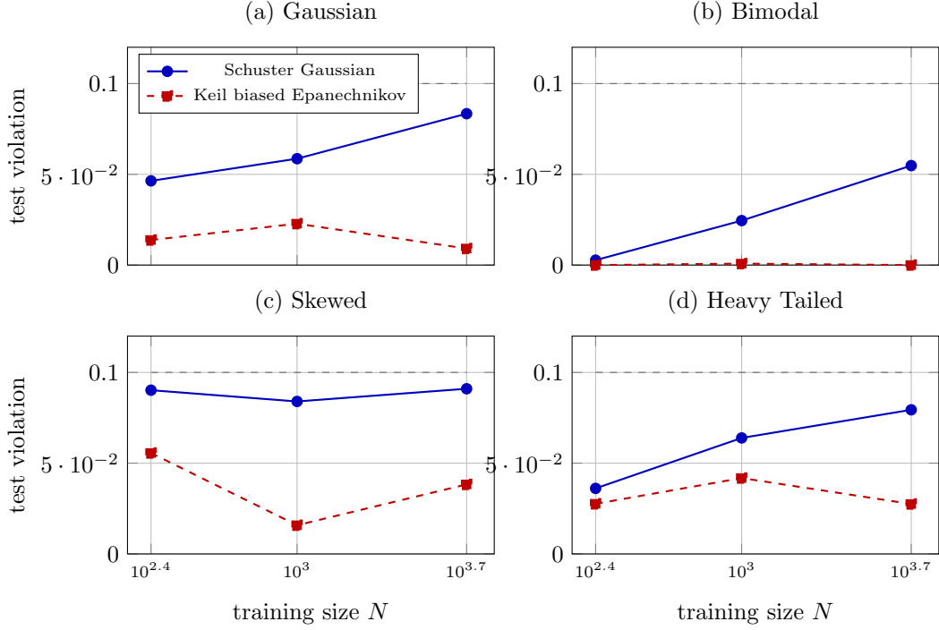
Figure 29: Paper-aligned static sequence. Lines show held-out violation for the Schuster Gaussian scaling and the Keil-biased Epanechnikov surrogate over nested training sizes. The dashed line is \varepsilon = 0.1 ; it is a target, not a confidence bound.
