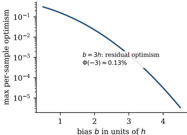
(b) The Gaussian kernel: no finite bias suffices
