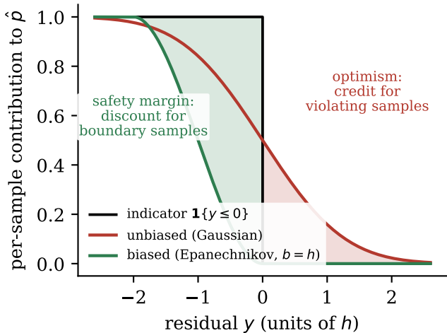
(a) The domination condition
