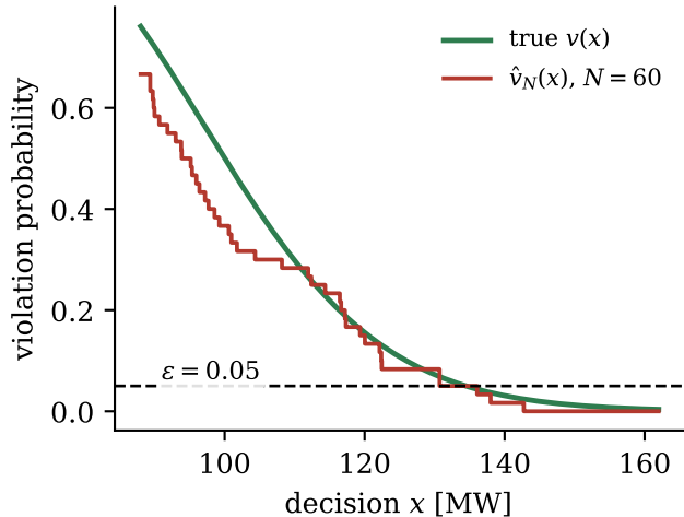
(a) The estimator is a staircase
