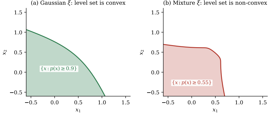
Figure 7: Convexity boundary for the computed bilinear constraint \xi^\top x \leq 1 . The Gaussian panel has a convex 0.9 probability level set, as follows from its Gaussian second-order-cone representation. Replacing the law by a two-component Gaussian mixture produces the non-convex 0.55 level set.
