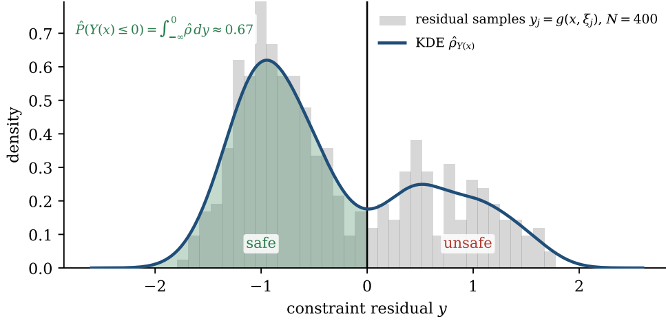
Figure 5: Residual-space estimation at a fixed decision, illustrated with 400 synthetic residual samples. A KDE smooths the histogram, and its mass on the shaded half-line estimates the safe probability. The residual samples change when the decision changes.
