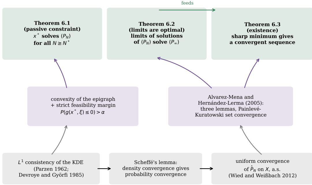
Figure 20: The architecture of the convergence theory of Schuster (2025). The statistical foundation (bottom row) is classical: L^1 consistency of the kernel estimator, upgraded to probability convergence by Scheffé’s lemma and to almost-sure uniform convergence on the feasible set under the conditions surveyed by Wied u. Weißbach (2012). Two analytical engines (middle row) convert statistical convergence into optimization statements: a convexity-of-epigraph argument with a strict feasibility margin, and the optimization-convergence theorem of Alvarez-Mena u. Hernández-Lerma (2005) verified through three lemmas. The three theorems (top row) divide the labor: exactness where the constraint is passive, optimality of limits, and existence of convergent solution sequences.
