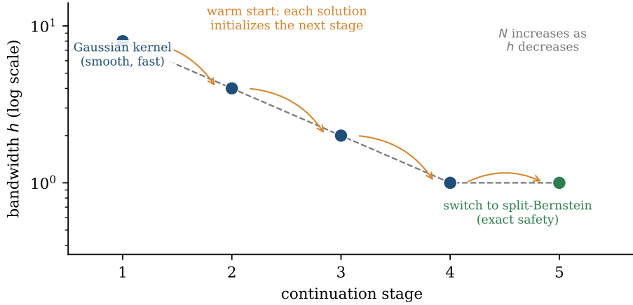
Figure 19: The bandwidth-continuation and kernel-switching schedule of Keil u. Rao (2021). Early stages use a large bandwidth and the fast Gaussian kernel, producing a benign landscape and a cheap solution; each stage’s solution warm-starts the next as the bandwidth shrinks and the sample size grows; the cited final stage switches to the split-Bernstein kernel; that literature step is not executed by the local runner. The homotopy stabilizes the solver and avoids the numerical difficulty of attacking a small-bandwidth, nearly nonsmooth constraint from a cold start.
