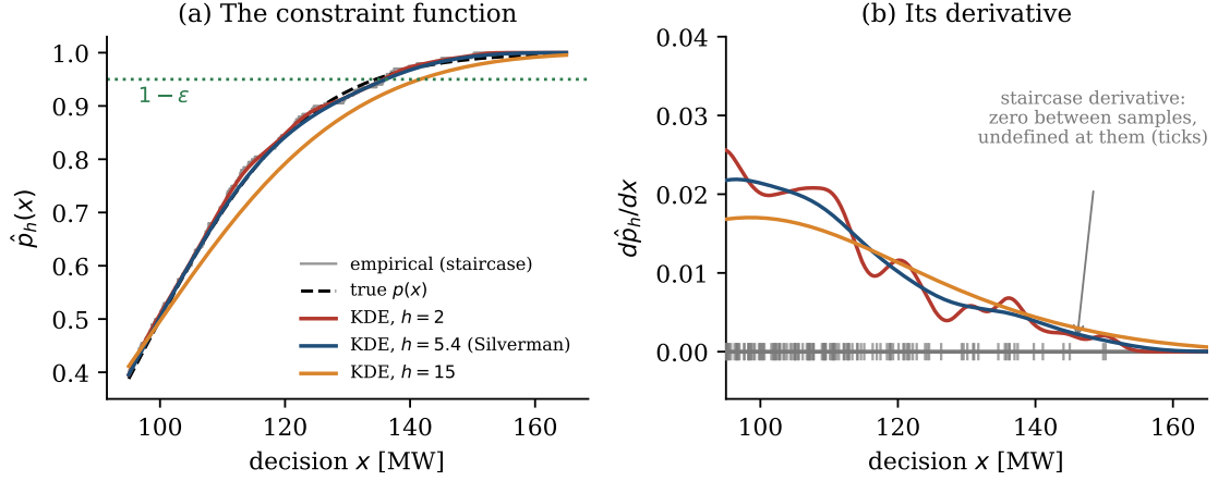
Figure 13: What the reformulation hands the solver, illustrated with a standalone lognormal scalar diagnostic ( N = 200 samples; this figure is not generated from the dispatch ledger). (a) The empirical staircase, the true probability p(x) , and the KDE constraint \hat{p}_h(x) at three bandwidths: small h tracks the staircase including its noise, Silverman’s h = 5.4 tracks the truth, and large h distorts the curve and shifts the feasibility boundary where it crosses 1 - \varepsilon . (b) The derivatives. The staircase derivative is zero between samples and undefined at them (ticks on the axis); the KDE derivative is an analytically available density estimate that gives the solver usable directional information at every x .
