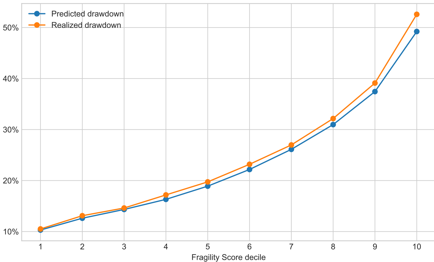
Positive drawdown magnitude
